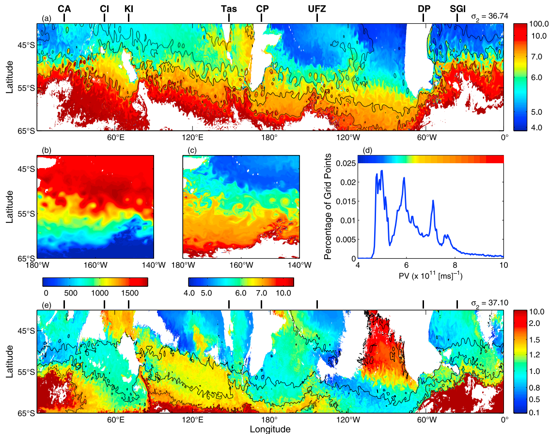
Figure 1. (a) Snapshot of potential vorticity PV ( \times 10^{-11} [\text{ms}^{-1}] ) on the \sigma_2 = 36.74 potential density surface in the Southern Ocean of the eddy-resolving OFES model. Land and isopycnal depths shallower than 100 m are colored white. Contours indicate isopycnal depth, with the 500, 1000 and 1500 m isolines plotted. (b) Isopycnal depth (m) over the region 180°W to 140°W and (c) an expanded view of PV in this region. (d) Probability density function of PV values in Figure 1c, normalized by the mean PV; the non-linear colorscale in Figures 1a and 1c is mapped onto the abscissa. (e) Snapshot of PV on the \sigma_2 = 37.10 potential density surface. Contours indicate the 1000, 2000 and 3000 m isolines of isopycnal depth. Markers above Figure 1a indicate key topographical features: CA, Cape Agulhas; CI, Crozet Island; KI, Kerguelen Island; Tas, Tasmania; CP, Campbell Plateau; UFZ, Udintsev Fracture Zone; DP, Drake Passage; SGI, South Georgia Island.
