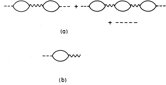
FIG. 1. (a) Diagrammatic representation of the conductivity due to the collective mode. (b) The matrix element M .
