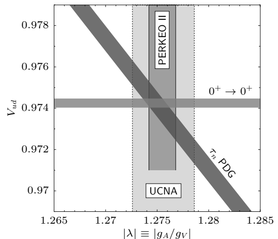
FIG. 3. The light quark weak coupling V_{ud} vs. \lambda . V_{ud} = 0.97425(22) from 0^+ \rightarrow 0^+ decays and the neutron lifetime \tau_n = 880.1(1.1) s are from PDG 2012 [33]. Values of \lambda are the UCNA result from this paper, and the PERKEO II combined result \lambda = -1.2755(13) from [32].
