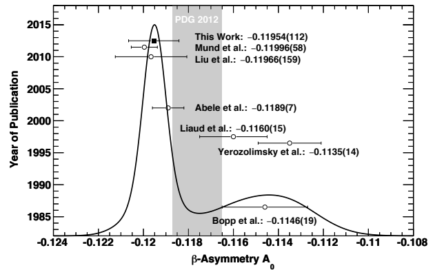
FIG. 2. Ideogram of values for A_0 from this work (filled square) and recent measurements (open circles) [7, 9, 28–32], arranged by year of publication. To account for correlated systematic errors in sequential measurements, the ideogram (solid curve) was constructed using the combined result from [31] and [32] of -0.11951(50) reported in [32], and the combined result of [7, 9] and this work of -0.11956(110) , as discussed in the text. The gray band indicates the PDG 2012 average value of A_0 = -0.1176(11) [33], which includes the results of [7, 9, 28–31], but does not include [32] or the work reported here.
