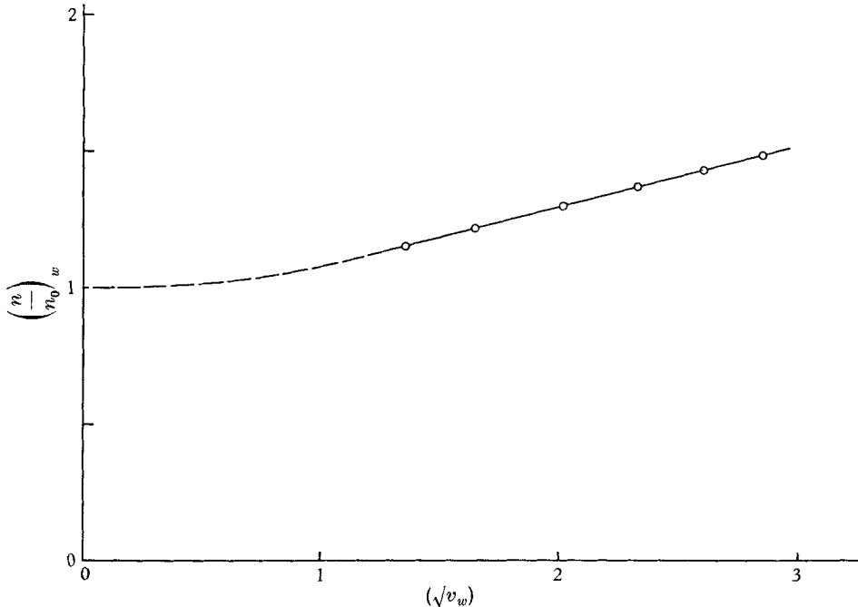
FIGURE 2. Typical hot-wire calibration. Data are for wire 1 with probe on outer cylinder at zero pitch, +15^\circ yaw (cf. figure 1 (b)). Ordinate is Nusselt number, normalized with free-convection value before extrapolation to wall. Abscissa is square root of relative velocity (in ft./sec) evaluated at surface of inner cylinder.
