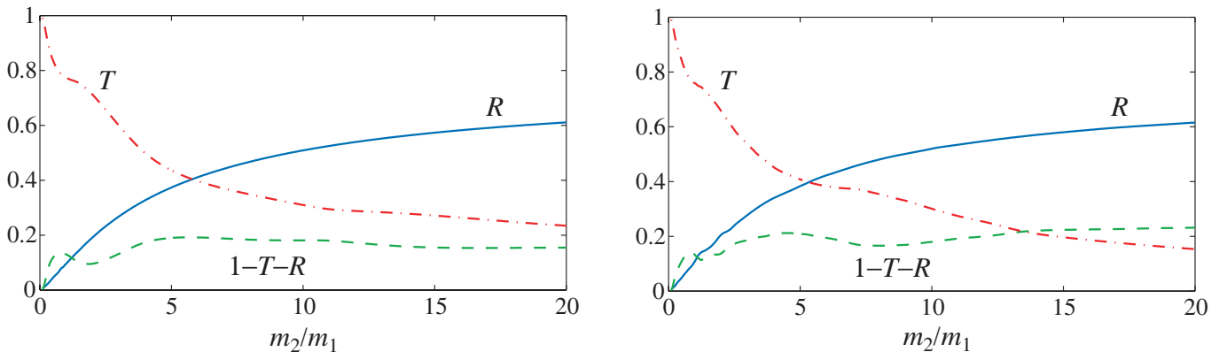
FIG. 8: The same diagnostics as those of Fig. 3 are shown here (transmitted T , reflected R and trapped 1 - T - R fractions of the energy) as a function of the mass ratio, but now for the case of two adjacent mass defects (left) and that of three adjacent mass defects (right).
