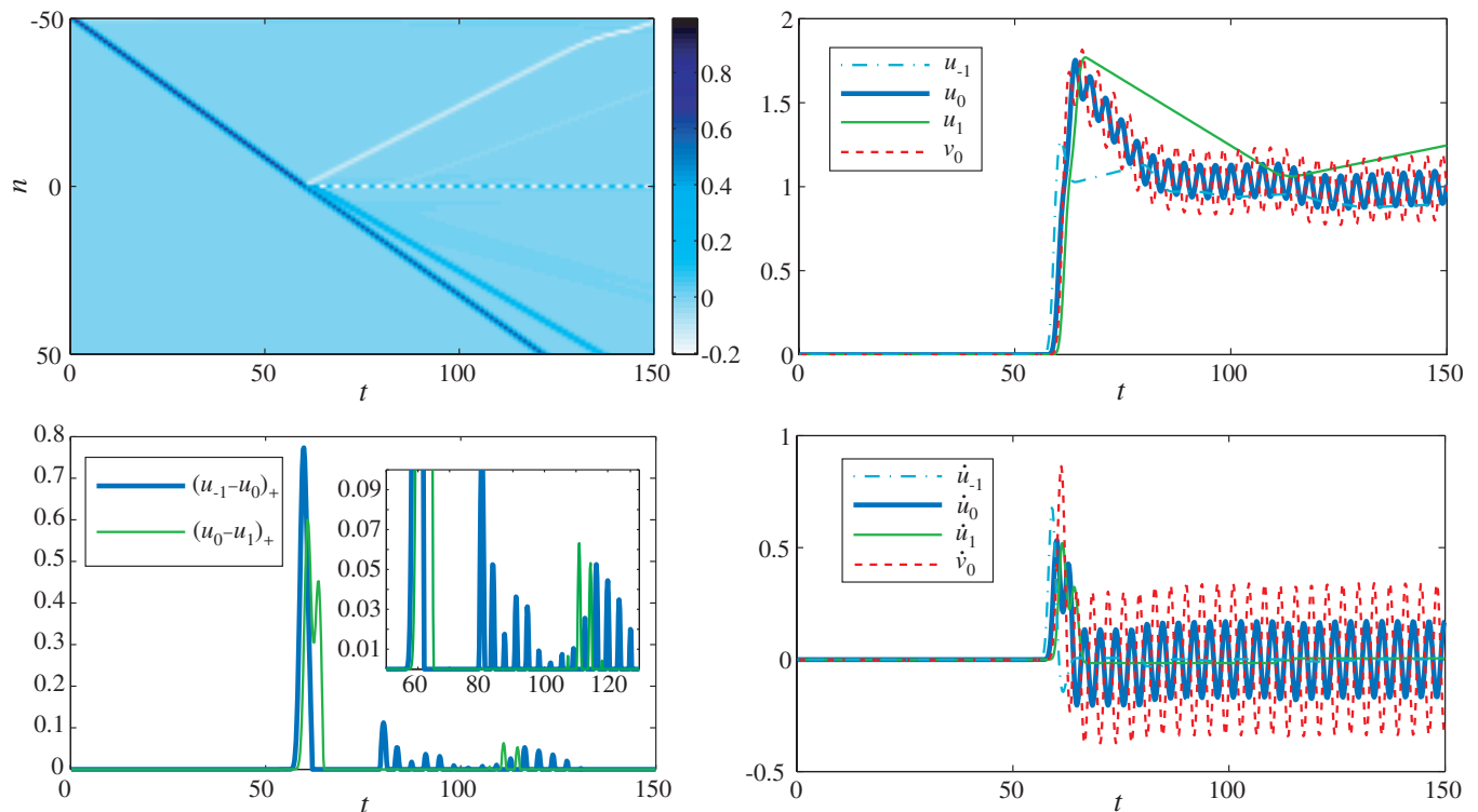
FIG. 7: The case of \epsilon = 0.5 , close to the value at which the maximal trapping occurs. The same diagnostics as for \epsilon = 0.1 in the case of Fig. 4 are shown. In this case the results reveal vibration over the fast scale of both u_0 and v_0 at the defect site and formation of only a second wave traveling to the right.
