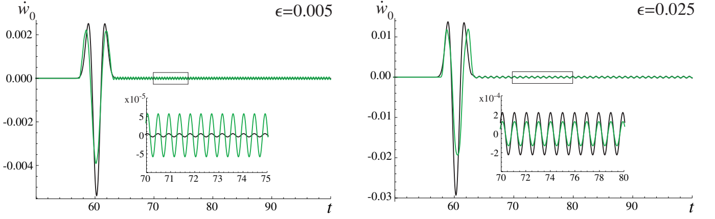
FIG. 9: The time derivative of the difference w_0(t) = u_0(t) - v_0(t) given by the direct numerical computation (black) and the analytical approximation (green) for \epsilon = 0.005 and \epsilon = 0.025 . The insets zoom in on the regions inside the rectangles.
