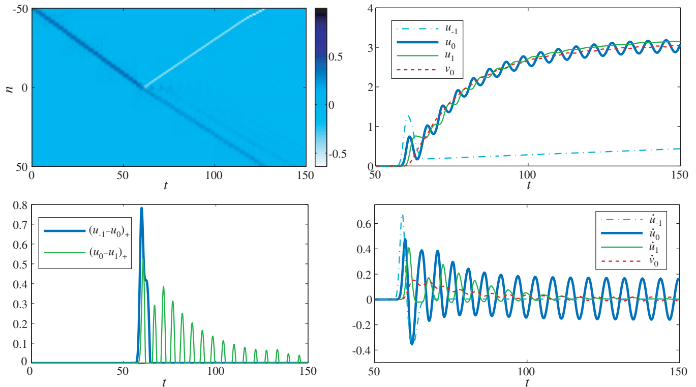
FIG. 6: The same properties as for the Fig. 4 are illustrated but now for the case of \epsilon = 10 . Here, it is the lighter mass m_1 executing the fast scale oscillations, while opening a gap from the site to its left and presenting a cascade of alternating gap openings and compression events with its right neighbor which, in turn, lead to the successive emission of progressively smaller amplitude (and thus slower) waves within the solitary wave train that emerges in the space-time contour plot.
