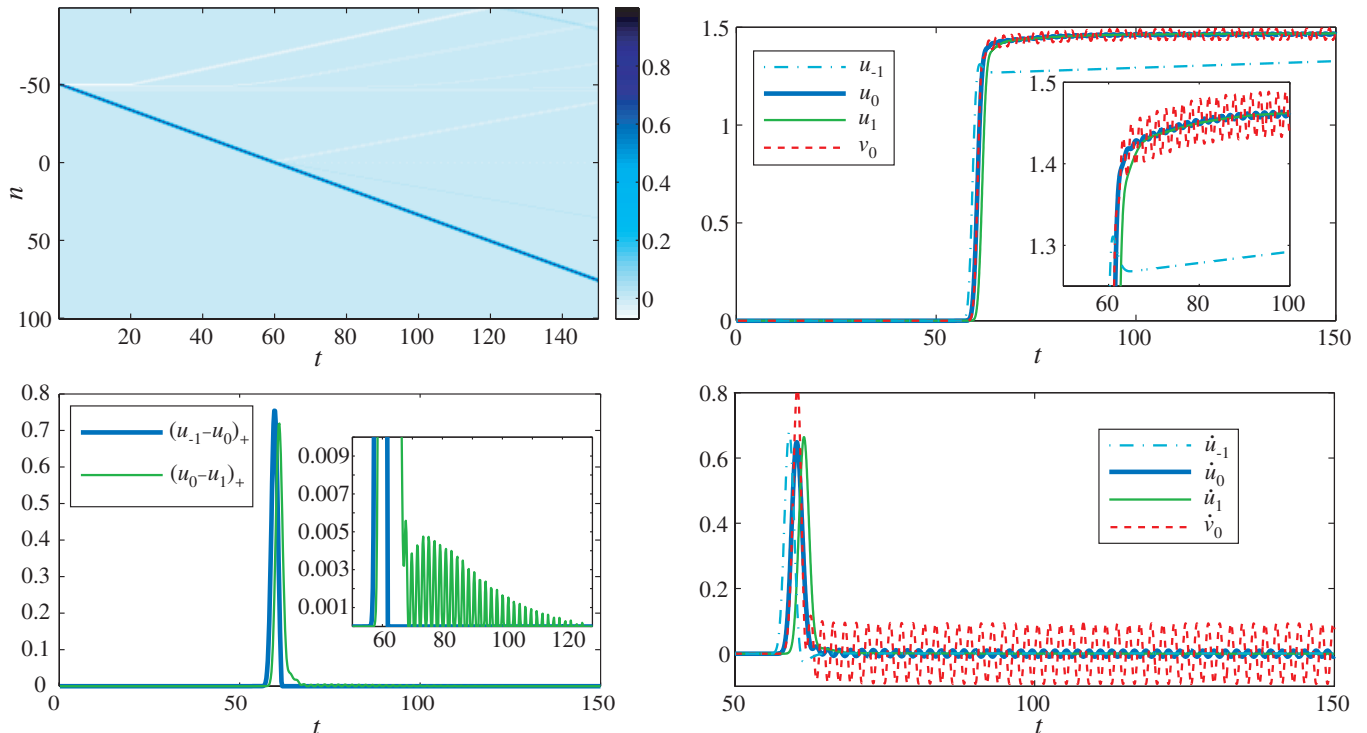
FIG. 4: The results of simulations at \epsilon = 0.1 . The top left panel presents the space-time ( n - t ) evolution of the contour plot of the field \dot{u}_n(t) . The thick blue and green lines in the bottom left panel show the quantities (u_{n-1} - u_n)_+ and (u_n - u_{n+1})_+ , respectively, to give a sense of when (after the impact) gap openings arise. The top right panel presents the displacements of the central sites; cyan dash-dotted line corresponds to u_{-1}(t) , thick blue solid to u_0(t) , green solid to u_1(t) and red dashed to v_0(t) . The same pattern is followed for the corresponding velocities at the bottom right plot.
