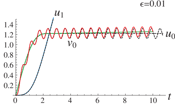
FIG. 11: Comparison of the numerical solution of (16), (17) at \epsilon = 0.01 (colored solid curves) and the two-timing approximation up to O(\epsilon) (black dashed curves).
