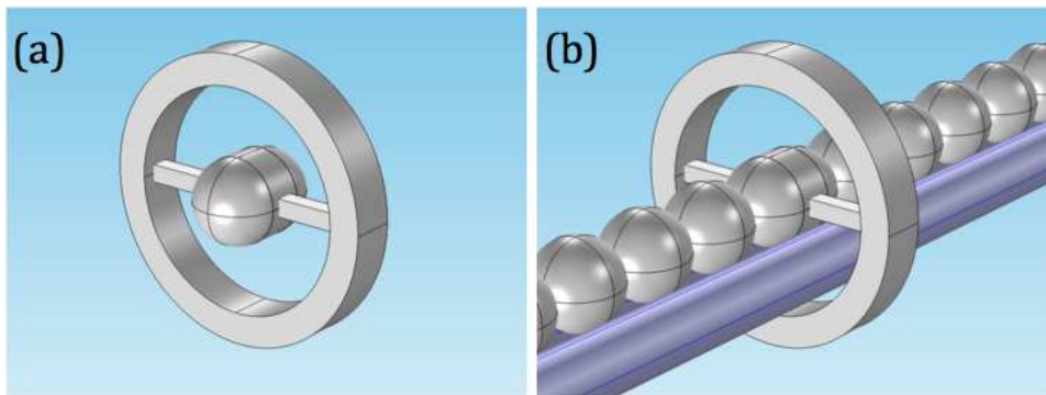
FIG. 2: Suggested experimental implementation of the mass-with-mass defect. (a) Defect bead with the ring resonator that provides the mass-with-mass. (b) Part of the suggested experimental setup containing the MwM defect.
