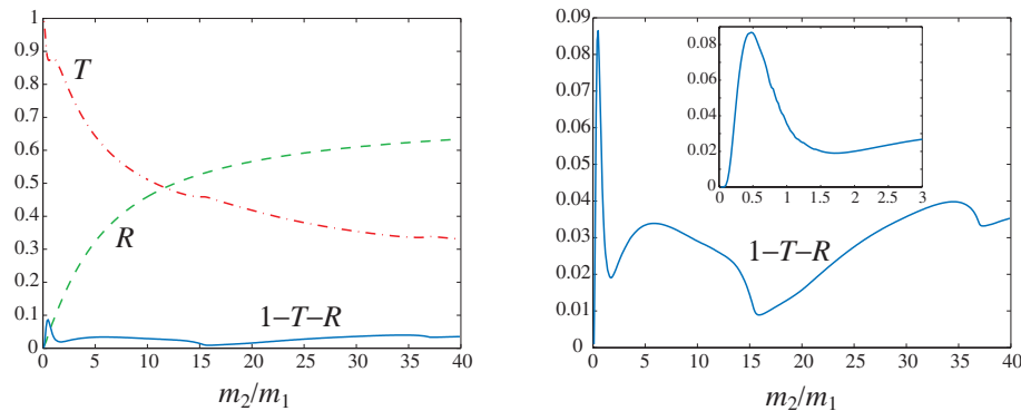
FIG. 3: Left panel: the different fractions of the energy are plotted as a function of the mass ratio \epsilon = m_2/m_1 . Right panel: trapped portion of the energy. The transmitted energy fraction T of the right part of the chain is presented by the red dash-dotted line, the reflected part of the energy R is given by the green dashed line, while the non-vanishing (for \epsilon > 0 ) trapped fraction of the energy is shown by the blue solid line.
