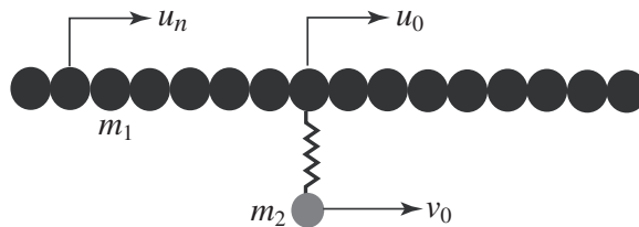
FIG. 1: Diagram of a granular chain containing a mass-with-mass defect.
