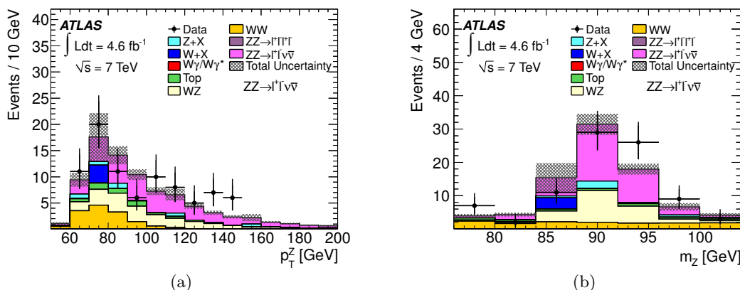
Figure 7. (a) Transverse momentum p_T^Z and (b) mass m_Z of the two-charged-lepton system for the ZZ \rightarrow \ell^+\ell^-\nu\bar{\nu} selection. The points represent the observed data and the histograms show the prediction from simulation. The shaded band shows the combined statistical and systematic uncertainty on the prediction.
