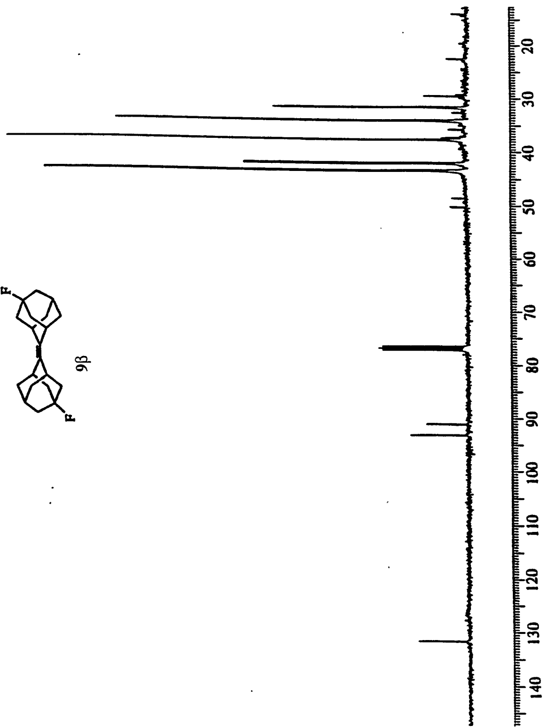
13 C NMR of 9β.
