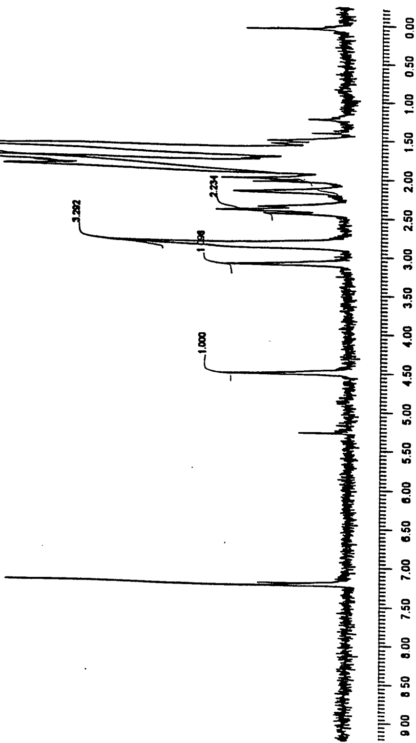
1 H NMR of 4(Br).
