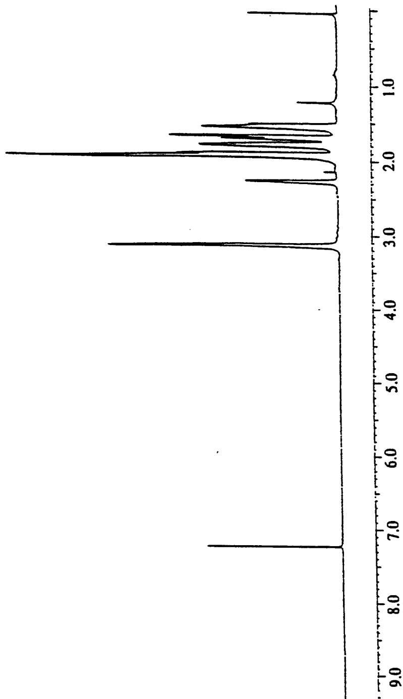
^1\text{H} NMR of 9 \alpha , 9 \beta mixture.
