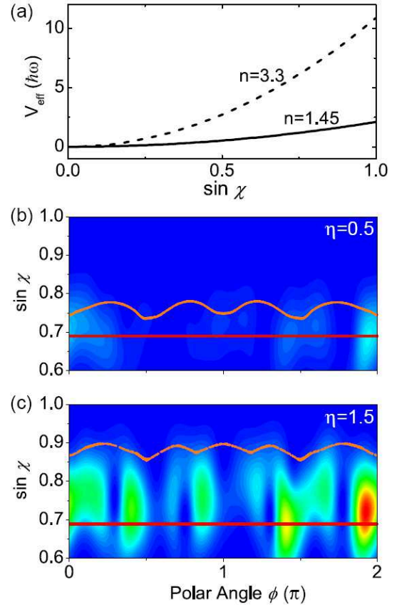
FIG. 6: (Color online) (a) Effective potential V_{\text{eff}} against \sin \chi . The solid and the dashed curves correspond to the cases of silica ( n=1.45 ) and GaAs ( n=3.3 ) microcavities, respectively. (b)-(c) Husimi projections of the excitation state inside the cavity at non-resonant frequency with the deformation parameter \eta of the cavity setting as 0.5 and 1.5, respectively. These two figures are plotted in the same scale. Orange dotted curves and red solid lines denote KAM tori and critical-refraction lines.
