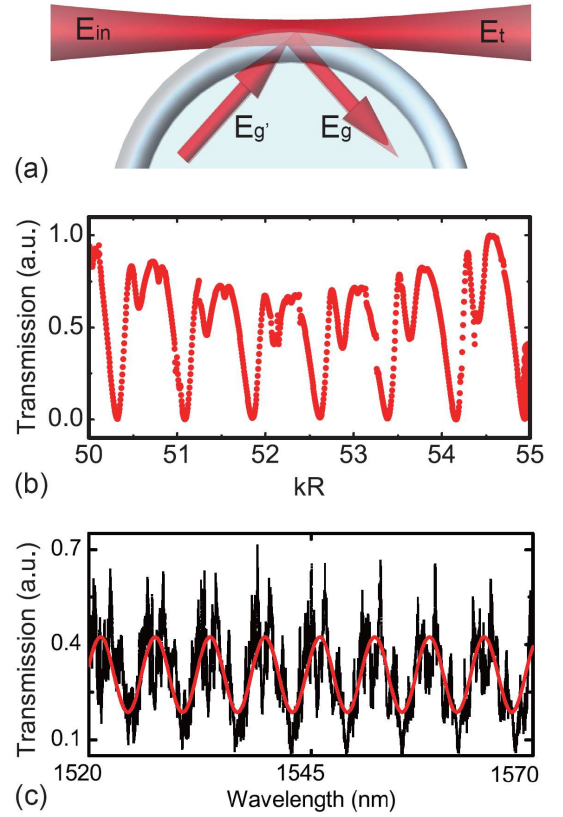
FIG. 3: (Color online) (a) The schema of the scattering process described by Eq. 17. (b) Stimulated transmission spectrum of the free-space excitation process obtained by boundary element method. (c) Experimental spectrum (black) and the fitted oscillations (red).
