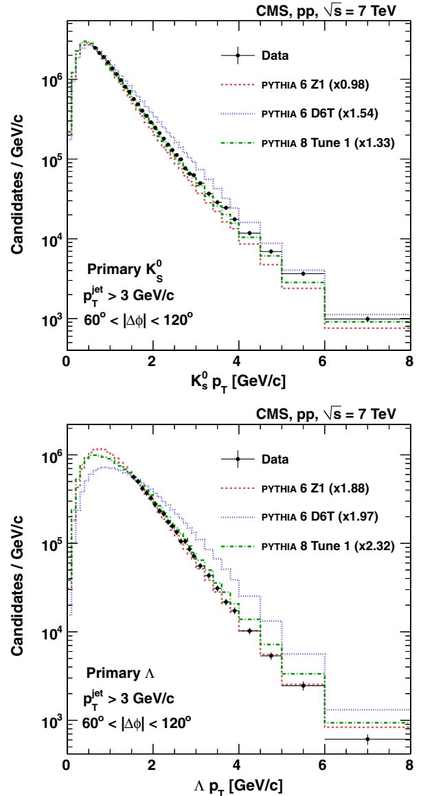
FIG. 6 (color online). V^0 p_T distributions corrected for selection efficiency and background without a correction to a leading reconstructed charged-particle jet, in the region transverse to a leading reconstructed charged-particle jet with p_T > 3 GeV/c, compared to predictions from different PYTHIA tunes (top: K_S^0 ; bottom: \Lambda ). Error bars indicate the quadratic sum of the statistical and systematic uncertainties. Simulations are normalized to the first p_T bin in the data, with normalization factors given in parentheses.
