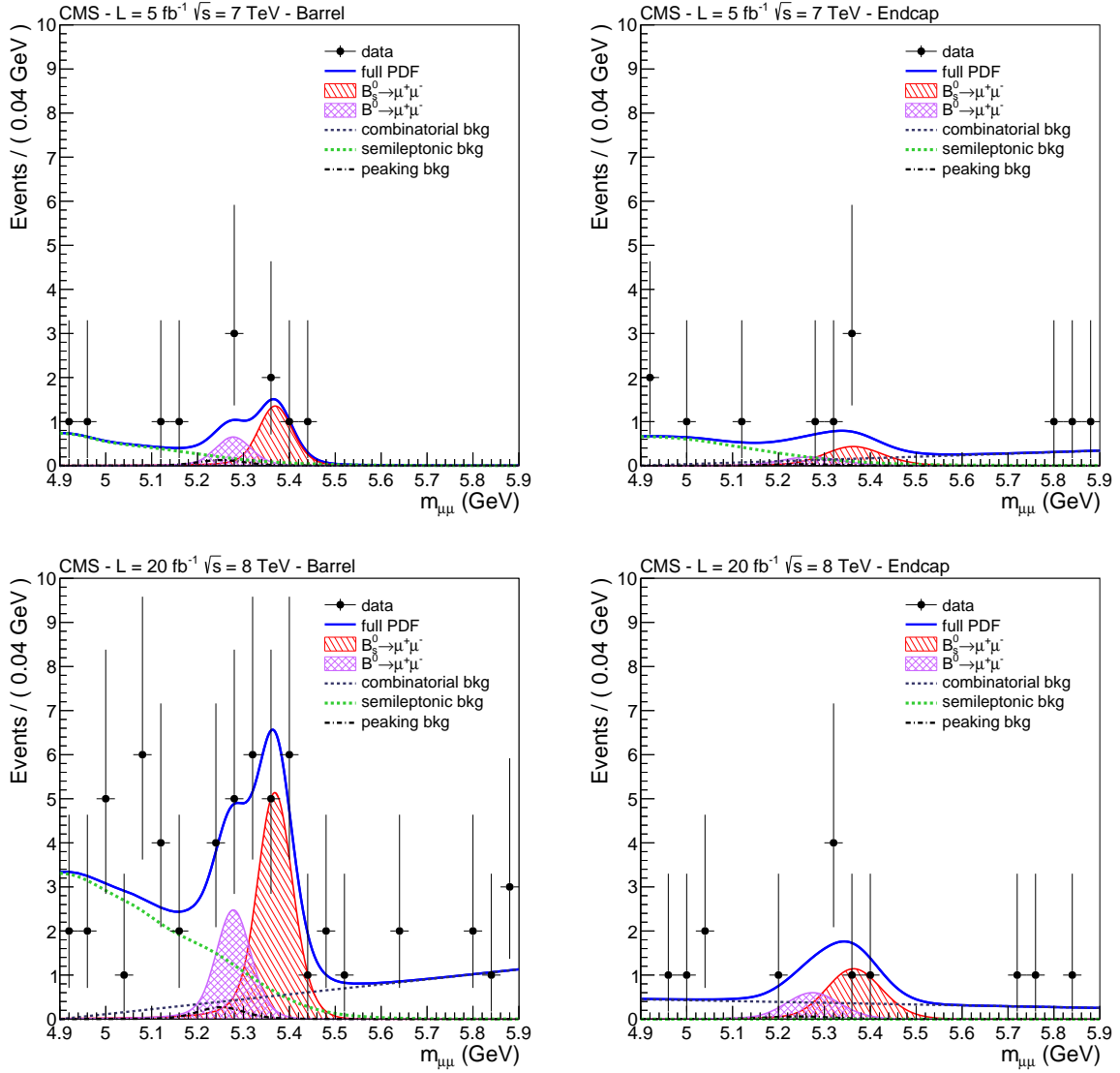
Figure 2: Results of the fit to the dimuon invariant mass distributions with the 1D-BDT method for the barrel (left) and endcap (right) from the 7 TeV (top) and 8 TeV (bottom) data samples. The points are the data, the solid line is the result of the fit, the shaded areas are the two B signals, and the different dotted lines are the backgrounds.
