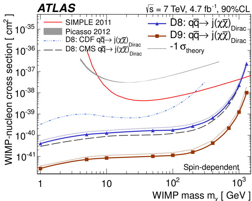
Figure 6. Inferred 90% CL ATLAS limits on spin-dependent WIMP-nucleon scattering. Cross sections are shown versus WIMP mass m_\chi . In all cases the thick solid lines are the observed limits excluding theoretical uncertainties, the observed limits corresponding to the WIMP-parton cross section obtained from the -1\sigma_{\text{theory}} lines in figure 4 are shown as thin dotted lines. The latter limits are conservative because they also include theoretical uncertainties. The ATLAS limits are for the four light flavours assuming equal coupling strengths for all quark flavours to the WIMPs. For comparison, 90% CL limits from the SIMPLE [73], Picasso [74], CDF [19], and CMS [21] experiments are shown.
