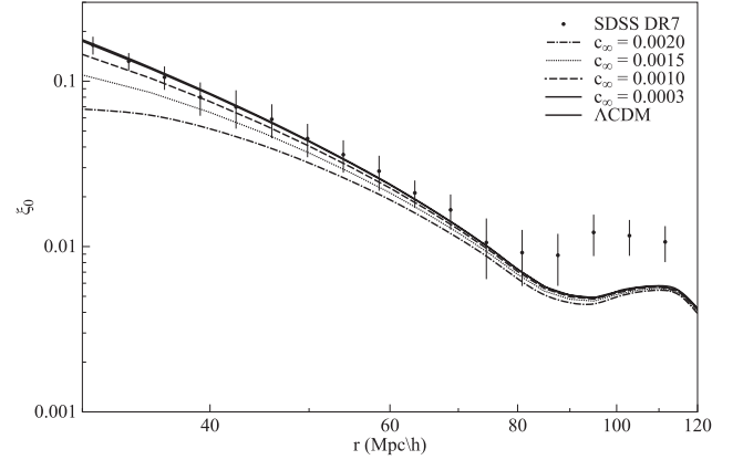
Figure 6. \xi_0 measured from SDSS DR7 and theoretical predictions for \Lambda\text{CDM} and UDM with different values of the speed of sound.
