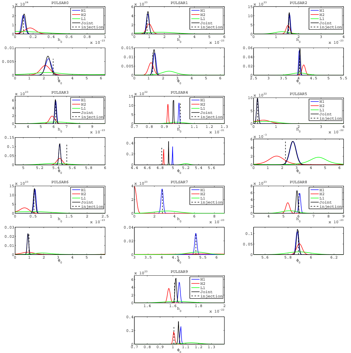
FIG. 7: The pdfs of h_0 and \phi_0 for 10 isolated pulsar injections into the LIGO detectors during S3. The anomaly seen in PULSAR7 is discussed in the text.
