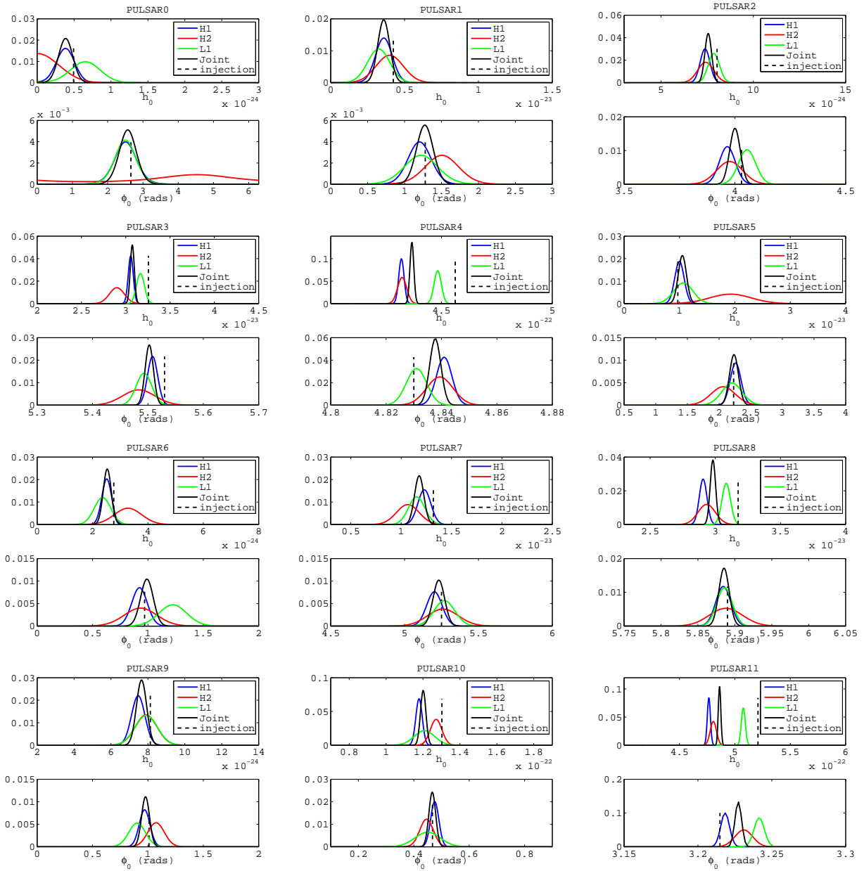
FIG. 8: The pdfs of h_0 and \phi_0 for 10 isolated and 2 binary pulsar injections into the LIGO detectors during S4.
