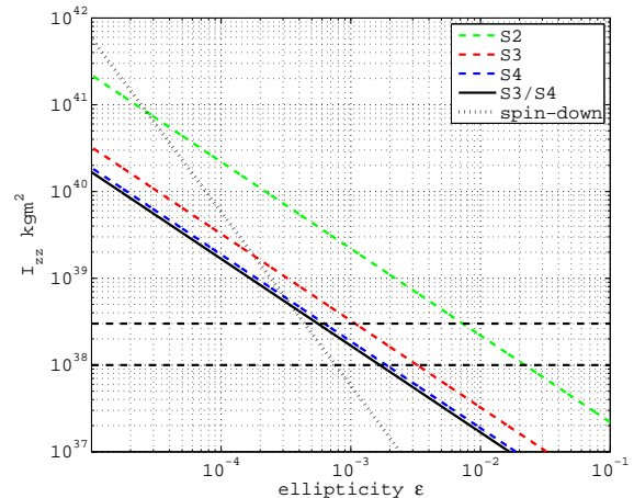
FIG. 6: The moment of inertia–ellipticity plane for the Crab pulsar over the S2, S3 and S4 runs. The areas to the right of the diagonal lines are the experimentally excluded regions. The horizontal lines represent theoretical upper and lower limits on the moment of inertia as mentioned in §VIB. Theoretical upper limits on the ellipticity are much more uncertain, the highest being a few times 10^{-4} .
