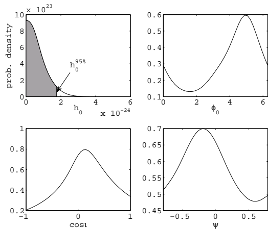
FIG. 2: The marginalised posterior pdfs for the four unknown pulsar parameters h_0 , \phi_0 , \cos i and \psi , for PSR J0024–7204C using the joint data from the three LIGO detectors over S3 and S4.
