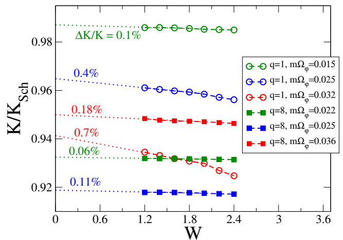
FIG. 3. Effect of the choice of width \varpi on the measured periastron advance. Shown are data for the three reference frequencies \Omega_{e/m/l} and for two exemplary runs: (q, \chi_1, \chi_2) = (1, 0, 0) and (q, \chi_1, \chi_2) = (8, 0.5, 0) . The symbols denote K_{\text{NR}}/K_{\text{Sch}} as measured with width \varpi indicated on the x -axis. The dotted lines denote fits indicating the extrapolation to zero width, \varpi \rightarrow 0 . The number next to each dotted line indicates the fractional change in K_{\text{NR}}/K_{\text{Sch}} between \varpi = 1.2 and \varpi \rightarrow 0 . For ease of plotting, the data for q = 8 and m\Omega_\varphi = 0.036 has been shifted up by 0.1.
