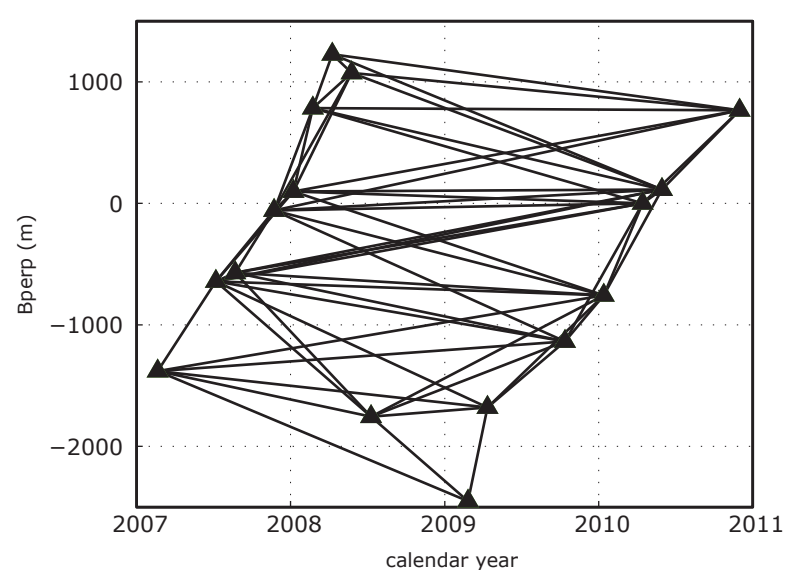
D) ALOS track 219, frame 700, Nifg=59, Nsar=16
