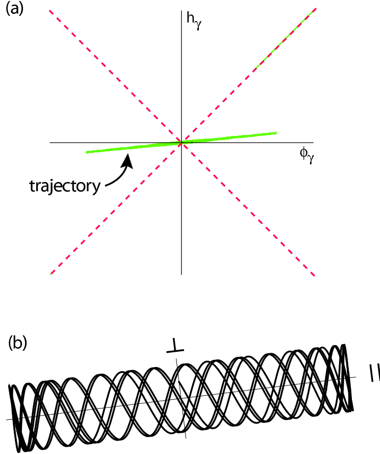
Fig.2: Figure (a) shows the back-and-forth trajectory of h_\gamma and \phi_\gamma in the \phi_\gamma - h_\gamma plane. Although the trajectory appears to be a straight slanted line when shown on this scale, Figure (b) is a blow-up that shows the trajectory to be more complicated. In this plane, the light-cone like lines correspond to the singularity in the Einstein frame, a_E^2 = (1/6)|\phi_\gamma^2 - h_\gamma^2| = 0 . In the left and right quadrants, the trajectory moves along an approximately fixed angle corresponding to a fixed Higgs value (constant h_c = h_\gamma/\phi_\gamma ), the current vacuum. As the trajectory moves towards the lightcone, the universe contracts ( a_E shrinks); crossing the lightcone corresponds to the big crunch/big bang transition; and moving away from the lightcone corresponds to expansion (growing a_E ). In Figure (b), the axis perpendicular to the trajectory ( \perp ) has been greatly expanded to show the combination of oscillations perpendicular and parallel ( \parallel ) to the trajectory, characteristic of the eternally cycling solution. From this figure it can be seen that cycles are quasiperiodic: similar but not identical, they explore an invariant torus in phase space as expected from the KAM theorem.
