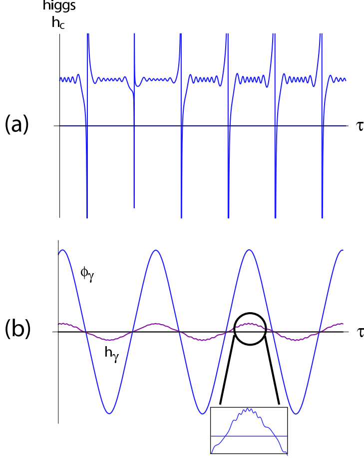
Fig.3: Graphs of the evolution of (a) the Higgs field ( h_c = h_\gamma/\phi_\gamma ), and (b) the scale factor ( a_\gamma = \phi_\gamma ) and h_\gamma , for the trajectory shown in Fig. 2. In (b), \phi_\gamma oscillates smoothly while the evolution of h_\gamma has barely detectable, high frequency oscillations (magnified in the inset) corresponding to the Higgs field oscillating back and forth in the potential well of the metastable phase. Note that, in (a), the Higgs oscillates around a fixed value (the current vacuum) for most of a cycle and then pops to large values up to the Planck scale during the crunch/bang transition. When the spikes in (a) cross \pm 1 (the Planck scale, beyond the range shown here), the lightcone in Fig. 2a is being crossed, corresponding to a big crunch/big bang transition where a_E vanishes.
