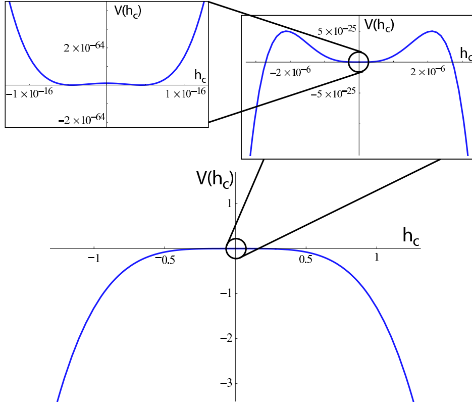
Fig.1: A sequence of expanded views of the metastable Higgs potential for the standard model suggested by recent LHC data. The Higgs field |h_c| and its potential energy density V(h_c) values are expressed in Planck units. The bottom figure shows that most of the Higgs field range corresponds to large negative energy density. The effective potential for |h_c| > 1 is subject to quantum gravity corrections, so the shape beyond |h_c| = 1 is unknown. The middle inset (upper right) shows the energy barrier whose height is nearly 25 orders of magnitude below the Planck density. The final inset (upper left) shows the current (spontaneous symmetry breaking) vacuum.
