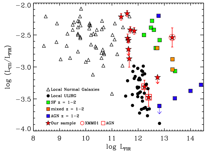
Figure 2. \log(L_{[\text{C II}]} / L_{\text{FIR}}) as a function of \log(L_{\text{FIR}}) for local normal and starburst galaxies (open triangles) from Malhotra et al. (2001), local ULIRGs (black filled circles) from Farrah et al. (2013) and Diaz-Santos et al. (2013), high-redshift ( 1 < z < 2 ) star-forming galaxies (green squares), mixed systems (orange filled squares) and AGNs (blue filled squares) from Stacey et al. (2010). Red stars denote the 12 intermediate redshift (U)LIRGs presented in this work (circled star is XMM01, squared stars denote AGNs). Note that L_{\text{FIR}(42.5\text{--}122.5 \mu\text{m})} = 0.63 \times L_{\text{IR}(8\text{--}1000 \mu\text{m})} .
