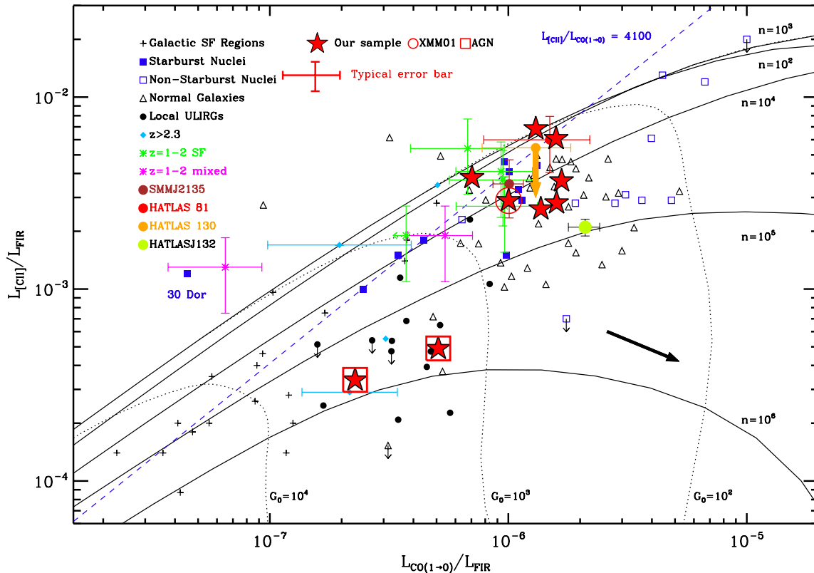
Figure 3. L_{[\text{C II}]} / L_{\text{FIR}} as a function of L_{\text{CO}(1-0)} / L_{\text{FIR}} for Galactic star-forming regions (crosses), local starburst nuclei (filled squares), local non-starburst nuclei (open squares), local normal galaxies (triangles), local ULIRGs (circles), redshift 1–2 sources (asterisks with error bars), high- z sources (cyan diamonds), adapted from Hailey-Dunsheath et al. (2010). Herschel lenses are from: SMMJ2135 (Ivison et al. 2010), HATLAS 81 and HATLAS 130 (Valtchanov et al. 2011), HATLASJ 132 (George et al. 2013). Red asterisks denote the present sample (circled star is XMM01, squared stars denote AGNs). The typical error bar shown refers to our sample only. Overplotted are the PDR model values for \eta and G_0 from Kaufman et al. (1999). The plot is based on observed values and is intended as a first order diagnostic tool, hence does not include any correction. The black arrow indicates the direction that all data points in the plot will shift when corrections are applied (see text).
