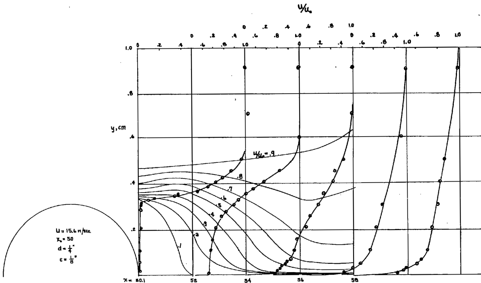
FIGURE 17b.- VELOCITY PROFILES DOWNSTREAM FROM A LARGE ROUGHNESS ELEMENT.
