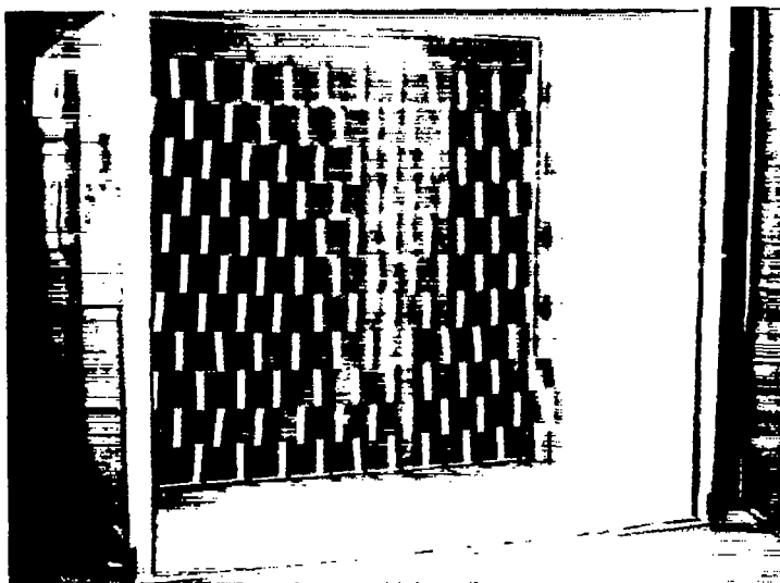
Figure 5.- Method of mounting paper strips to create artificial turbulence in the tunnel.
