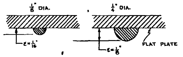
FIGURE 2c.- MOUNTING OF ROUGHNESS ELEMENTS.
