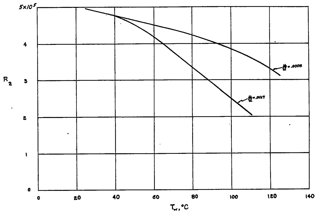
FIGURE 14. - EFFECT OF PLATE TEMPERATURE ON THE REYNOLDS NUMBER OF TRANSITION ( \nu_{\text{FREE STREAM}} ).
