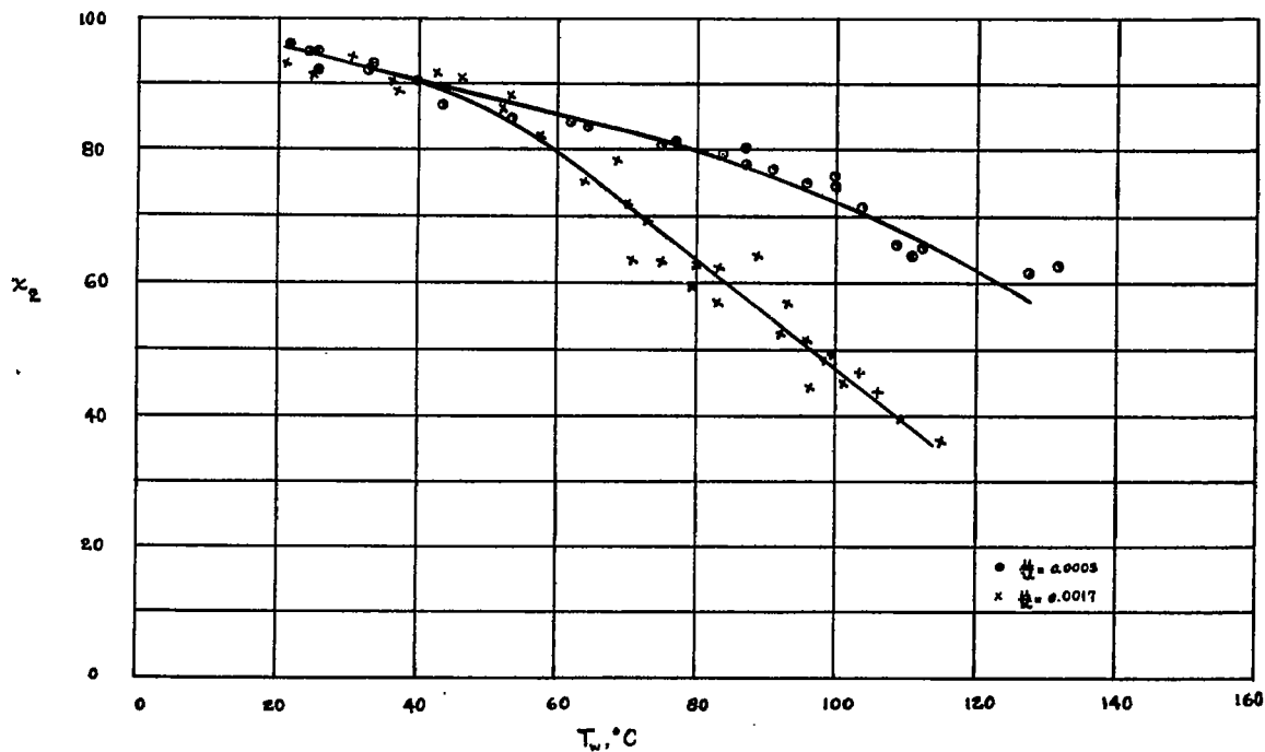
FIGURE 13. - EFFECT OF PLATE TEMPERATURE ON TRANSITION.
