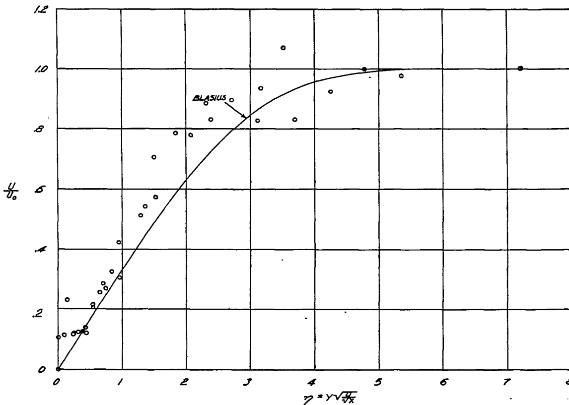
FIGURE 12a. — VELOCITY DISTRIBUTION IN THE BOUNDARY LAYER OF THE HEATED PLATE. UNPREDICTED PROFILE DUE PROBABLY TO SECONDARY FLOW.
