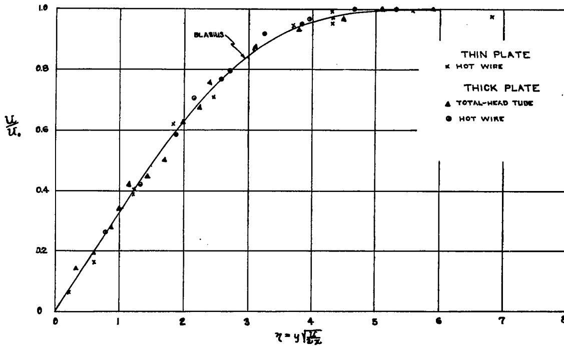
FIGURE 9.- VELOCITY DISTRIBUTION IN THE BOUNDARY LAYER OF THE UNHEATED FLAT PLATE.
