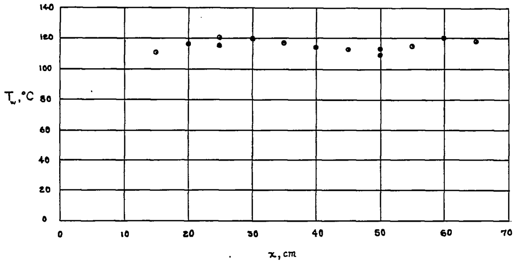
FIGURE 6. - TEMPERATURE DISTRIBUTION ALONG THE HEATED PLATE.
