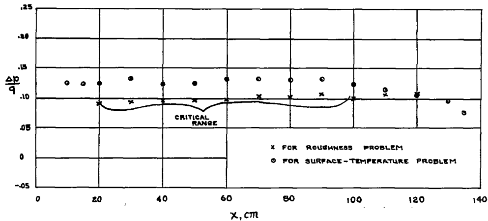
FIGURE 8. - PRESSURE DISTRIBUTION ALONG THE TEST PLATE.
