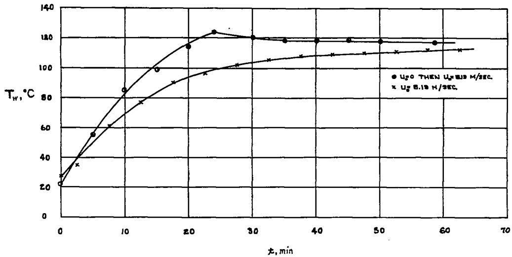
FIGURE 7. - TWO METHODS OF HEATING THE FLAT PLATE.
