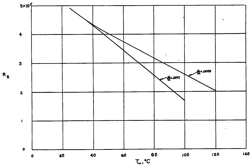
FIGURE 15. - EFFECT OF PLATE TEMPERATURE ON THE REYNOLDS NUMBER OF TRANSITION ( \nu_{\text{WALL}} ).
