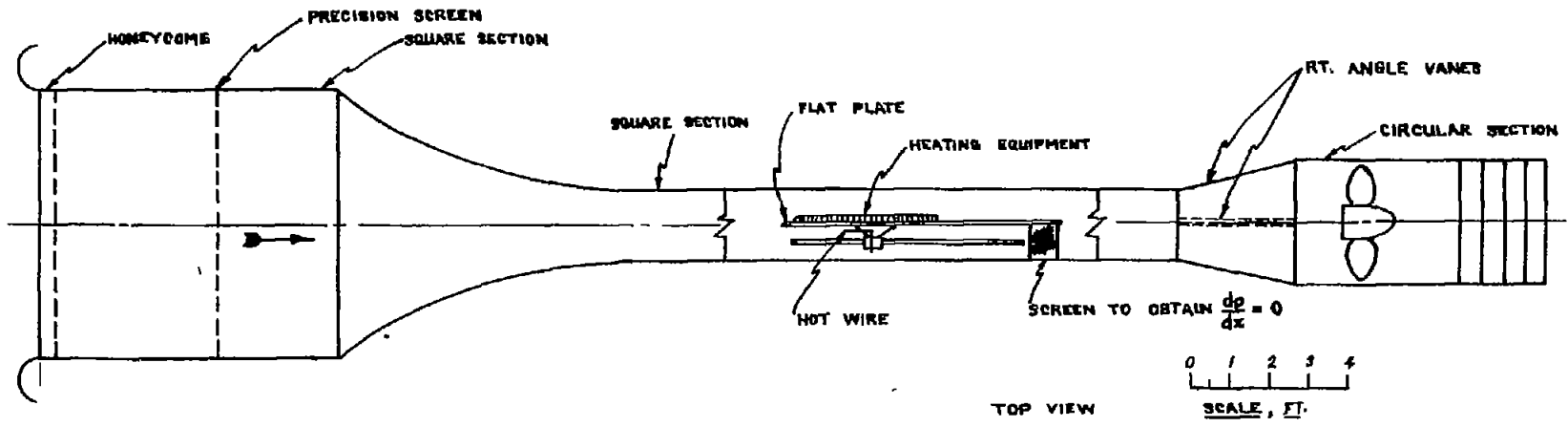
FIGURE 2a.- SCHEMATIC DIAGRAM OF THE WIND TUNNEL.
