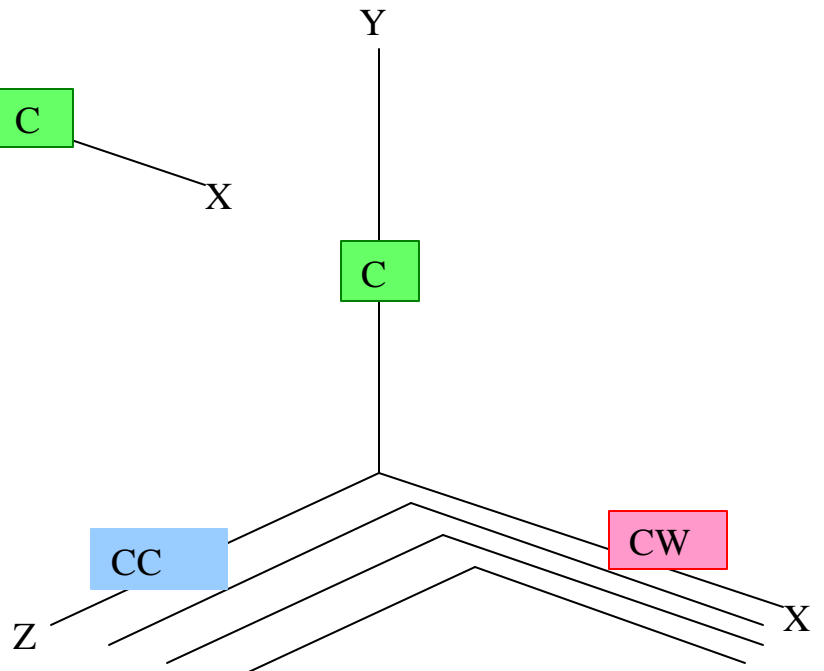
Type X and Z Preferences
