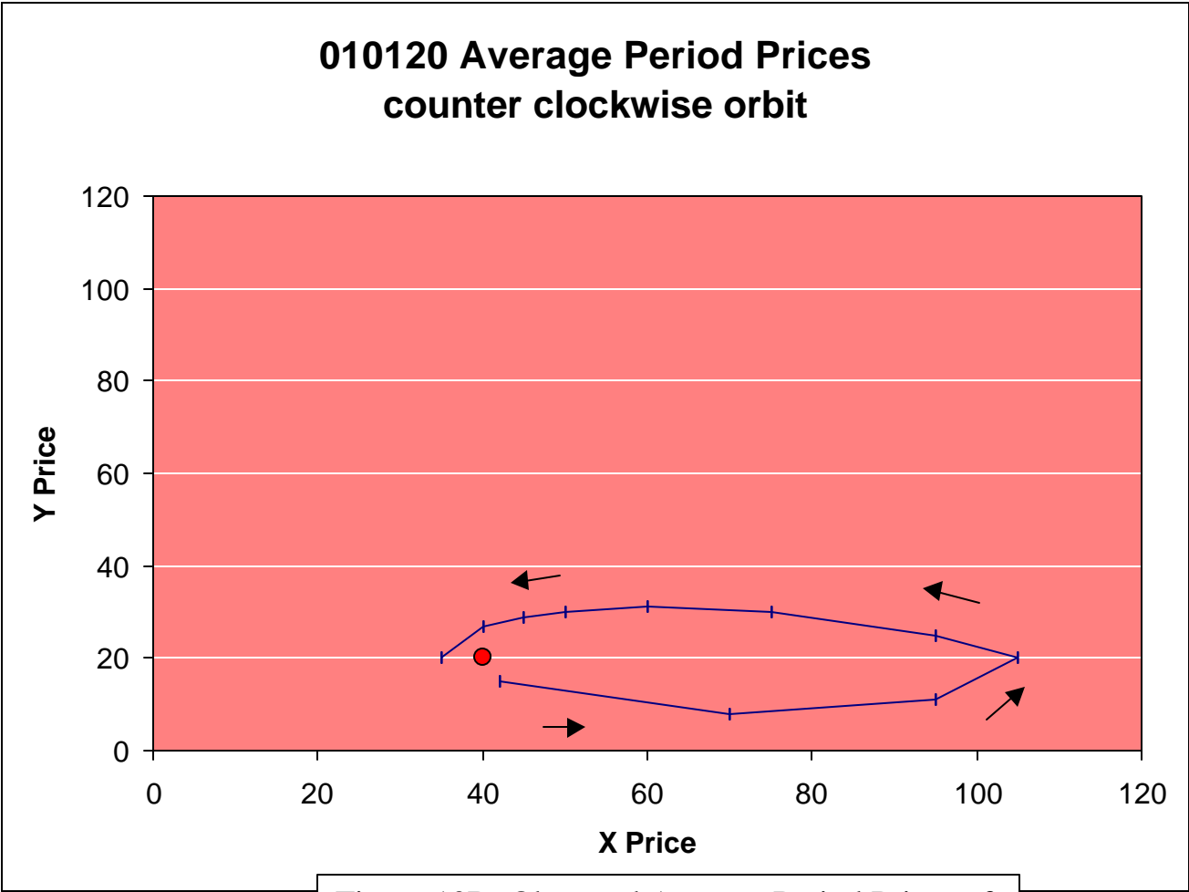
Figure 10B: Observed Average Period Prices of X and Y for all Periods, Counterclockwise Orbit Parameters
