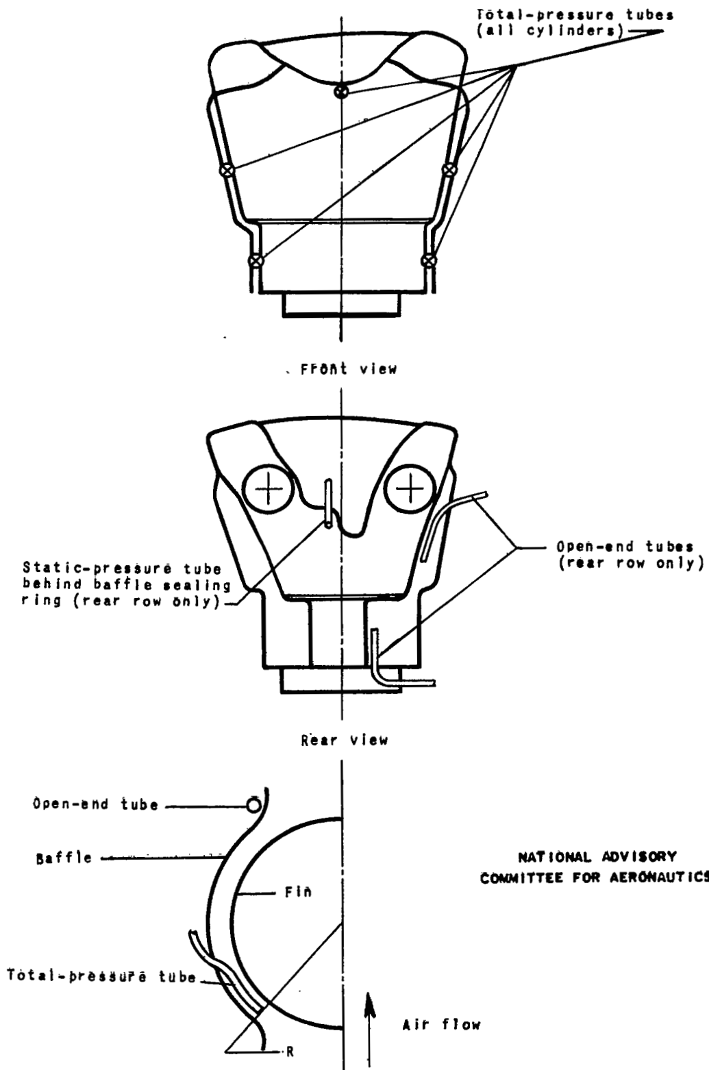
Figure 4. - Location of cooling-air pressure tubes.
