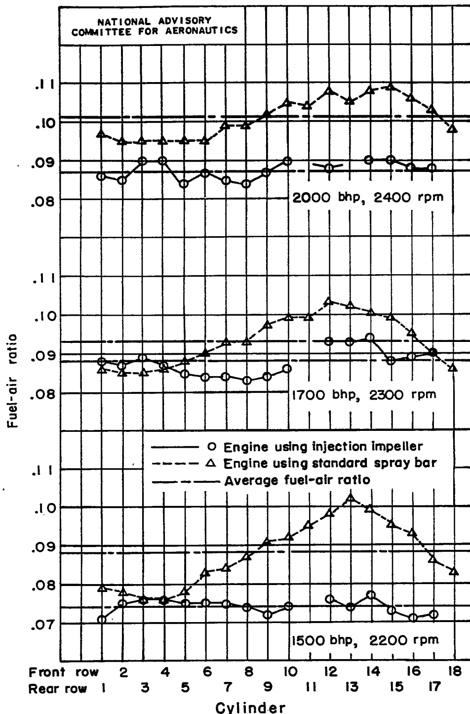
Figure 7.— Effect of NACA injection impeller on mixture distribution of engine at reduced fuel flows.
