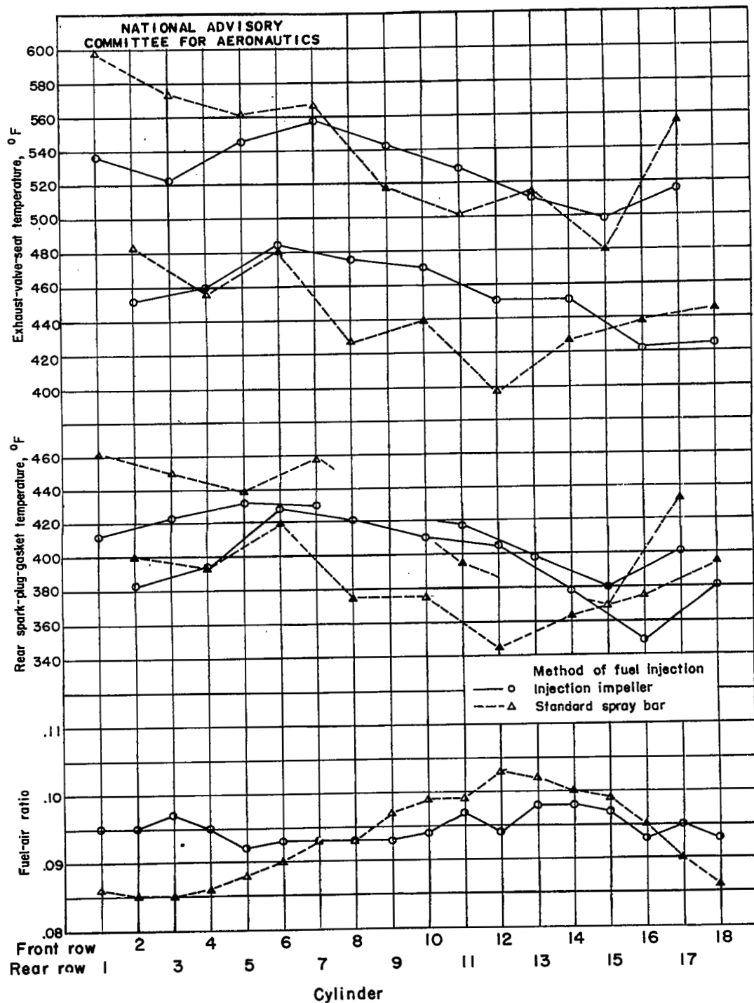
(c) Brake horsepower, 1700; engine speed, 2300 rpm.
