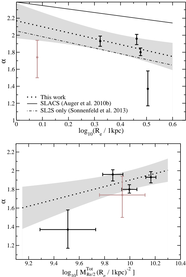
Figure 4. Correlation between total mass density profile slope, \alpha , and effective radius, R_e , ( top panel ) and average projected total surface mass density within R_e/2 ( bottom panel ). In both panels, the Sa lens J091305.0-005343, coloured with a grey data point, has been omitted in the straight line fit which is shown by the dotted line and grey shaded 1\sigma error envelope.
