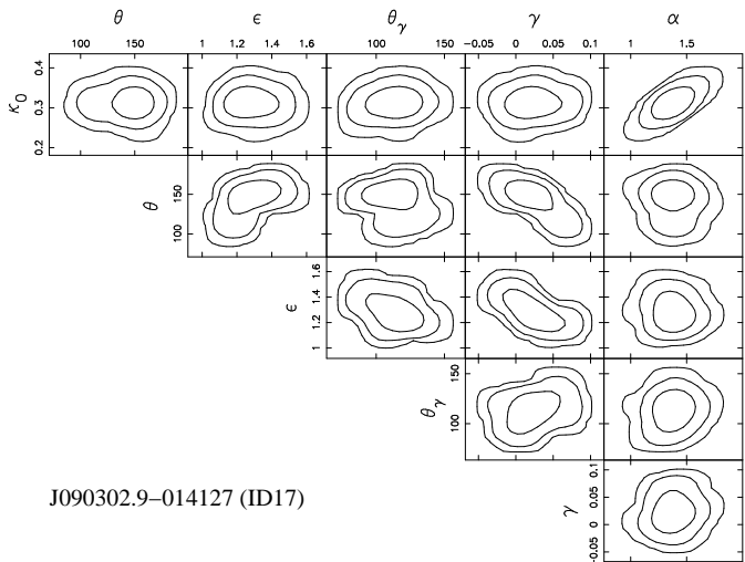
Figure A1. Parameter confidence limits. Contours show the 1, 2 and 3 \sigma single-parameter confidence regions for all parameter combinations, excluding the position centroid of the lens.
