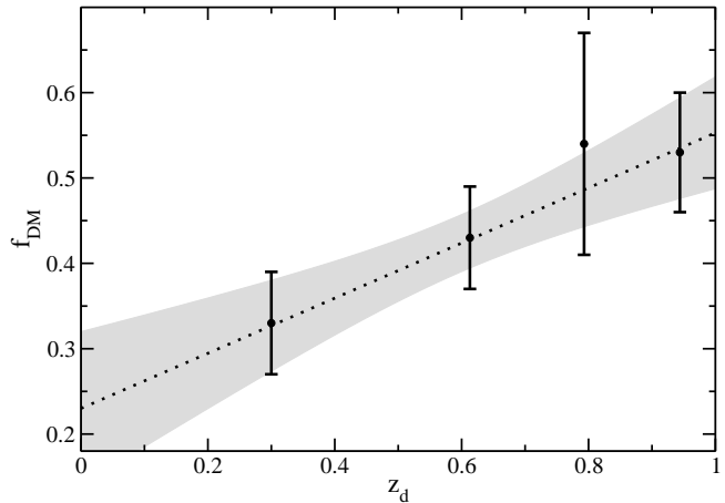
Figure 5. Variation of the fraction of dark matter within half the effective radius, f_{\text{DM}} , for a Salpeter IMF with redshift. The grey shading depicts the 1\sigma error region for the straight line fit.
