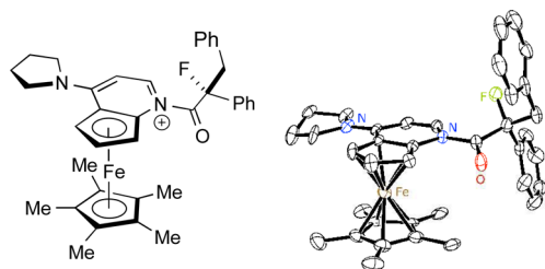
Figure 3. ORTEP diagram of N -acylated (+)- PPY* . Thermal ellipsoids are illustrated at the 35% probability level. For clarity, the carborane counteranion, the hydrogen atoms, the solvent, and the second molecule in the asymmetric unit are omitted, and only the major component of the disorder in the \text{Cp}^* group is shown.
