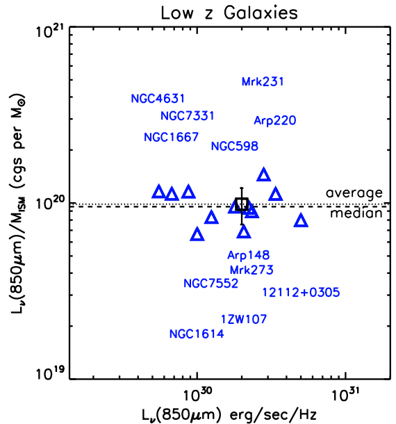
Figure 1. The ratio of L_\nu at 850\ \mu\text{m} to M_{\text{ISM}} is shown for a sample of low-z spiral and starburst galaxies from Dale et al. (2005) and Clements et al. (2010). The average and median values for the sample are shown by horizontal lines. The mean ratio shown by the error bars is 1.00 \pm 0.23 \times 10^{20} \text{ ergs sec}^{-1}\text{Hz}^{-1} M_\odot^{-1} . Typical uncertainties in the derived ISM masses are \pm 50\% due to variation in the CO to \text{H}_2 conversion factor.
