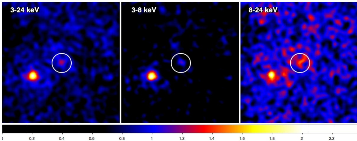
Figure 1. NuSTAR smoothed images of the source NuSTAR J033202–2746.8 at 3 – 24 keV (left), 3 – 8 keV (center), and 8 – 24 keV (right), from the FPMA and FPMB modules combined. The white circles have 30'' radius. The source is undetected down to a probability Prob = 4 \times 10^{-4} in the 3 – 8 keV band, but has a clear detection in the broader 3 – 24 keV energy band ( Prob = 10^{-9} ), and in the 8 – 24 keV band ( Prob \approx 4 \times 10^{-6} ).
