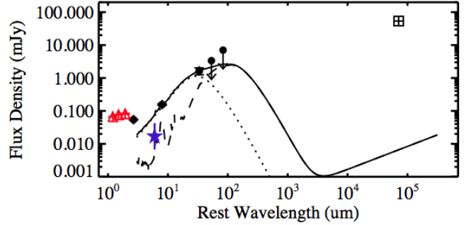
Figure 5. Infrared SED of NuSTAR J033202–2746.8, using Spitzer 8 and 24 \mu\text{m} data and Herschel 100, 160 and 250 \mu\text{m} data (black points) from the GOODS-H (Elbaz et al. 2011), PEP (Magnelli et al. 2013) and HerMES surveys (Oliver et al. 2012). In red triangles the Spitzer 3.6, 4.5 and 5.8 \mu\text{m} photometric points are also shown, while the open square represents the VLA radio flux density; these data points are not used to constrain the SED. The blue star represents the 6 \mu\text{m} luminosity predicted from the measured X-ray luminosity (2 – 10 keV) assuming the L_{6\mu\text{m}} - L_{\text{X}} relation by Lutz et al. (2004). The best-fitting SED (solid curve), the AGN component (dotted curve), and the star-formation component (dashed curve) are also shown. We note that at the excess of flux density at \lambda < 3 \mu\text{m} (red triangles) is probably due to emission from old stellar populations in the host galaxy. The SED fit was done fixing z = 2.00 (see Sect. 4.3).
