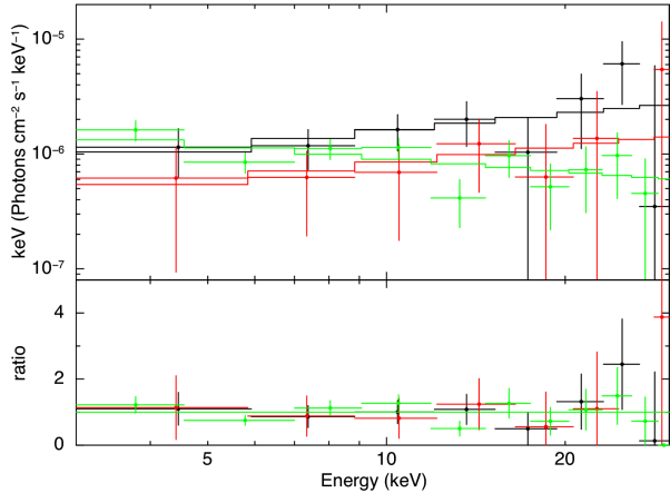
Figure 4. Comparison between the NuSTAR simulated spectrum (green), obtained assuming the best-fitting parameters resulting from fitting the XMM-Newton spectra with Model 1, and the real NuSTAR data for NuSTAR J033202–2746.8 (FPMA: black, and FPMB: red); the spectra have been rebinned for presentation purposes. The solid lines represent the power-law models fitted to the data. The bottom panel shows the ratio between the model and the data. The real NuSTAR spectra of NuSTAR J033202–2746.8 have a flatter spectral slope than that of the simulated spectrum, suggesting the need for a reflection component.
