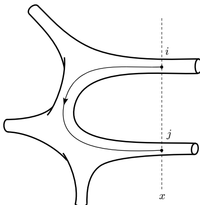
Figure 3. Period corresponding to domain wall interpolating between vacuum i and vacuum j of the theory at a given value of the SUSY parameter x .
