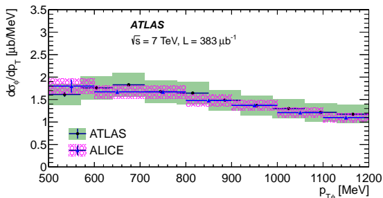
Fig. 5: The \phi(1020) -meson cross section as a function of p_{T,\phi} , extrapolated using PYTHIA6 to the kinematic region with 500 < p_{T,\phi} < 1200 MeV and |y_\phi| < 0.5 , is compared to the measurement by the ALICE Collaboration [3]. The error bars represent the statistical uncertainty and the boxes represent the quadratic sum of the statistical and systematic uncertainties. The 3.5% uncertainty on the luminosity is not included.
