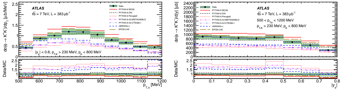
Fig. 4: The \phi(1020) \rightarrow K^+K^- cross section in the fiducial region, with 500 < p_{T,\phi} < 1200 MeV, |y_\phi| < 0.8 , p_{T,K} > 230 MeV and kaon momentum p_K < 800 MeV, as a function of p_{T,\phi} (left) and |y_\phi| (right). The error bars represent the statistical uncertainty and the green boxes represent the quadratic sum of the statistical and systematic uncertainties. The 3.5% uncertainty on the luminosity is not included. The data are compared to various MC expectations as described in the legends.
