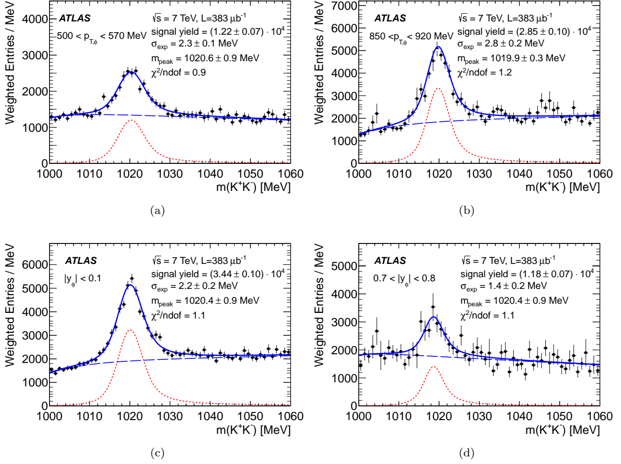
Fig. 3: Examples of invariant K^+K^- mass distributions in the data (dots) compared to results of the fits (solid lines), as described in the text, for (a) the lowest p_{T,\phi} bin, (b) one of the middle p_{T,\phi} bins, (c) the most central |y_\phi| bin and (d) most forward |y_\phi| bin. The dashed curves show the background contribution and the dotted red curves demonstrates the signal contributions, with parameters listed in the legend.
