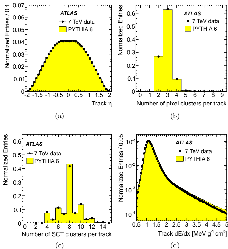
Fig. 2: Comparison between data (black dots) and MC simulation (histogram) for (a) track \eta , (b) number of pixel clusters assigned to the track, (c) number of SCT clusters assigned to the track and (d) the average track energy loss (see text). Statistical uncertainties are smaller than the marker size.
