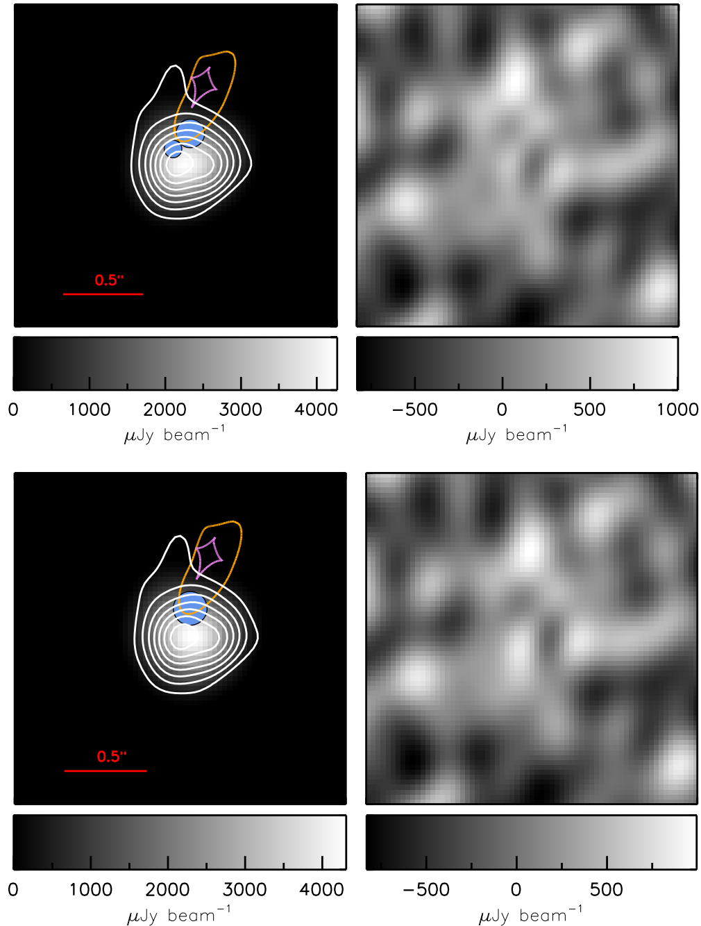
Figure 2. Top left: source and image planes of HFLS3 under the best-fit lens model with two components for the background source to describe HFLS3. In blue, we show the two components of HFLS3 in the source plane that are gravitationally magnified. The image plane involves the background grayscale color that is compared to the measured IRAM/PdBI 1.1 mm continuum emission shown with contours. The two lines are the critical line (orange) in the image plane and the lensing caustic (pink) in the source plane. Top right: residual map for the best-fit model showing the difference between observed IRAM/PdBI 1.1 mm continuum emission and the lens model output. Bottom left and right: lens model and residual for the case involving HFLS3 described by a single source (shown in blue). The lines and the residual intensity to the right are the same as top two panels.
