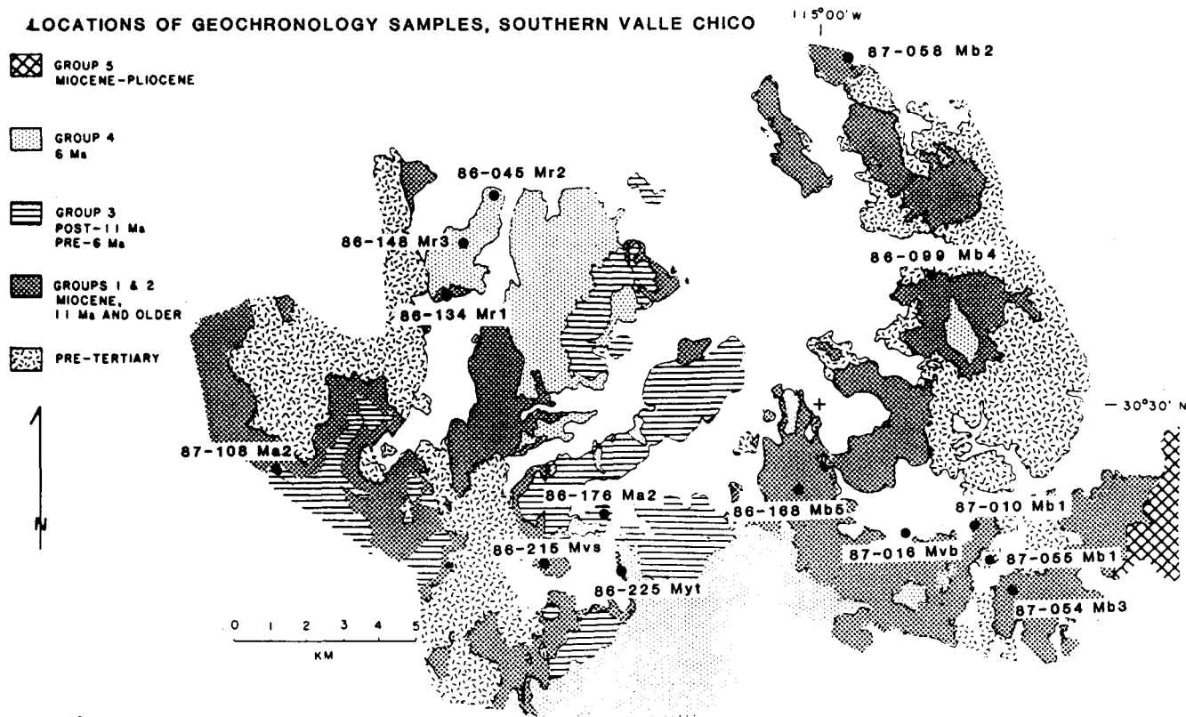
Fig. 3. Locations of geochronology samples (Tables 1 and 2). The VC- prefix in front of each sample ID number has been omitted. The 3- or 4-character code following the sample ID number is the abbreviation of the corresponding geologic map unit, discussed in text.
