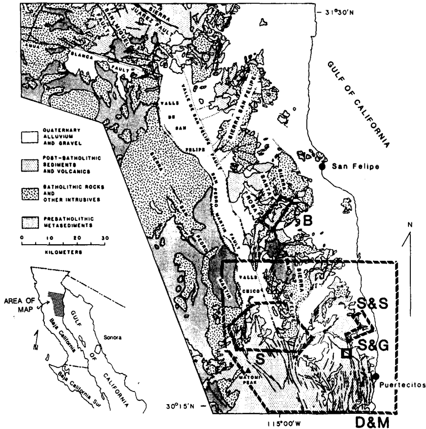
Fig. 1. Regional geologic map of part of northeastern Baja California, after Gastil et al. (1975). Areas discussed in the text are outlined: S = Stock (this study); B = Bryant (1986); S&G = Sommer and García (1970); D&M = Dokka and Merriam (1982).
