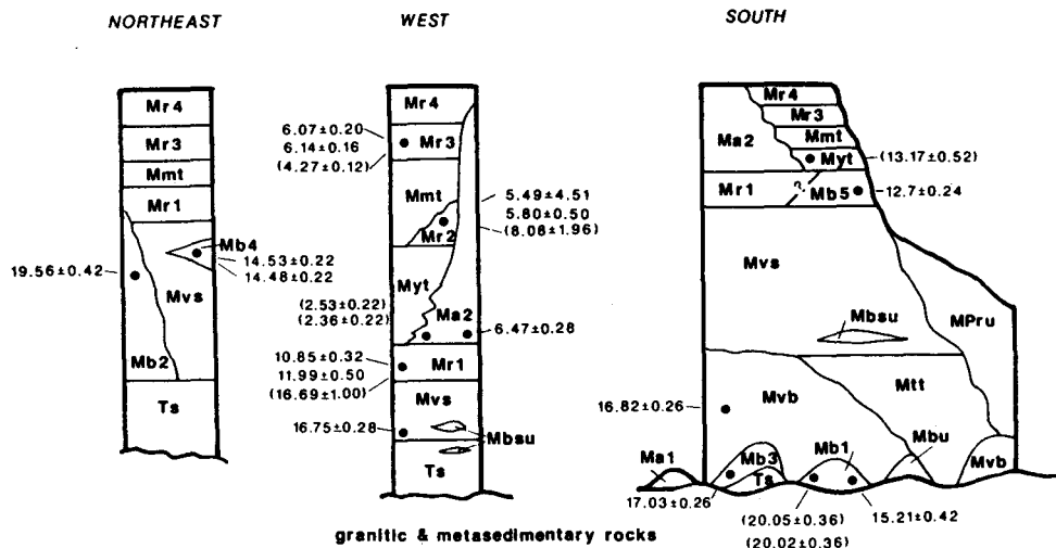
Fig. 4. Schematic stratigraphic columns, summarizing the depositional relationships of the units present in the northeastern, western, and southern parts of the mapped area. Dots show stratigraphic positions of dated samples, with the corresponding K/Ar or ^{40}\text{Ar} - ^{39}\text{Ar} total fusion ages. Suspect ages are in parentheses (see discussion of individual units in the text). Thicknesses are not to scale and angular discordances are not shown.
