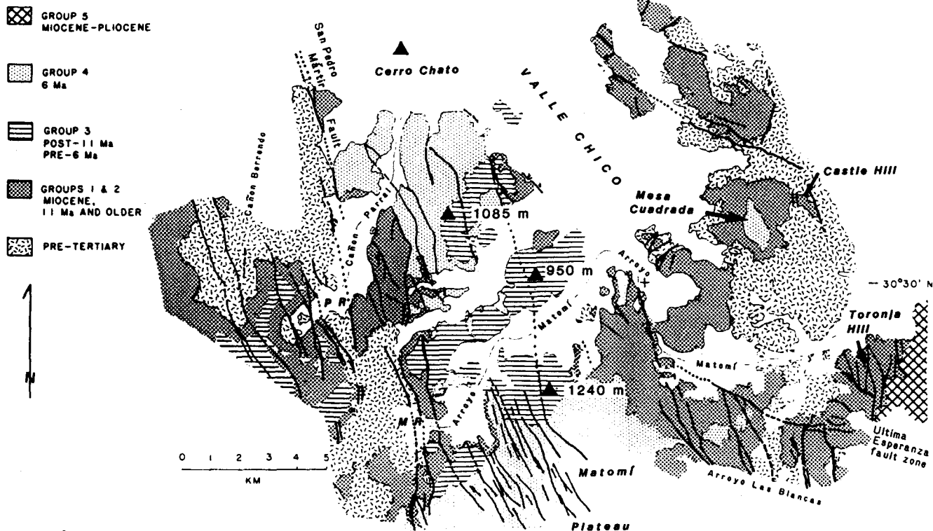
Fig. 2. Simplified geologic map of the study area, showing physiographic features mentioned in the text. Triangles with labeled elevations are the highest peaks of post-11 Ma, pre-6 Ma volcanoes. MR = Matomí Ranch; PR = Parral Ranch. Strata are grouped as discussed in the text. Pre-Tertiary rocks are granitic and metasedimentary rocks of the Peninsular ranges batholith.
