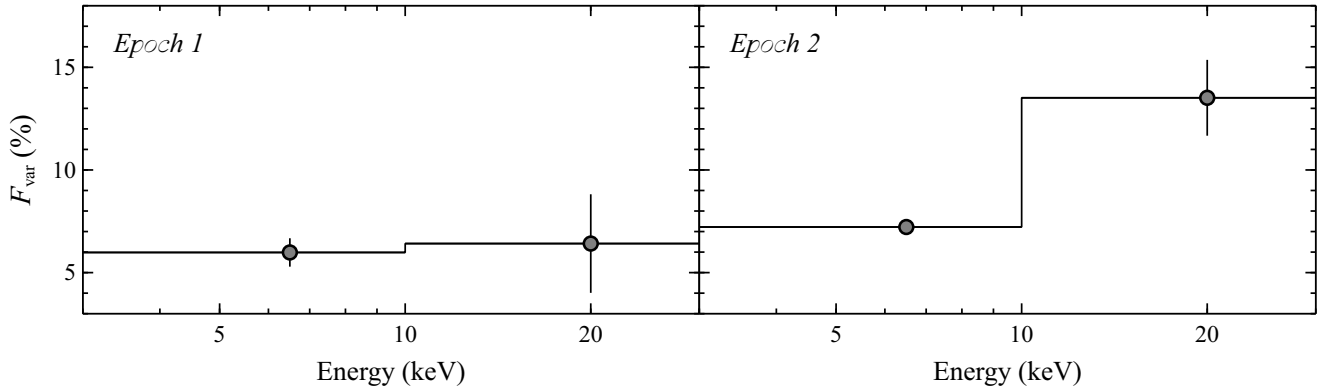
FIG. 8.— The fractional excess variability ( F_{\text{var}} ; covering frequencies 1.4 \times 10^{-5} - 10^{-3} Hz, i.e. 5–70 ks timescales) above and below 10 keV observed from Holmberg IX X-1 with NuSTAR during the two epochs (see section 4). There is tentative evidence for enhanced variability above 10 keV in the second epoch.
