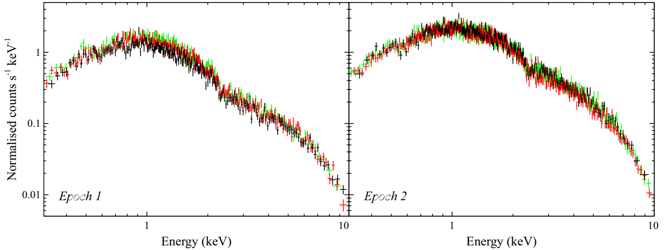
FIG. 2.— EPIC -pn spectra for the two sets of three observations of Holmberg IX X-1, the first taken in October ( left panel ; associated with NuSTAR observation 1) and the second in November ( right panel ; associated with NuSTAR observation 2). The black, red and green spectra show the first, second and third observations from each set of three. Although there is some mild flux variability displayed by the observations in each set, it is clear there is very little spectral variability.
