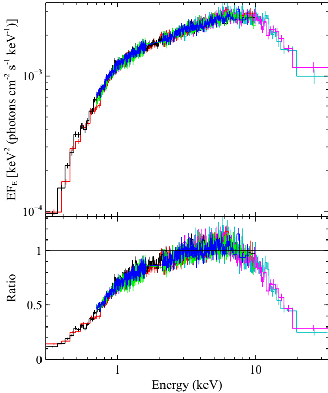
FIG. 4.— Top panel : The broadband X-ray spectrum displayed by Holmberg IX X-1 during epoch 1. All the data have been unfolded through the same model, which simply consists of a count spectrum that is constant with energy. Bottom panel : data/model ratio to the powerlaw continuum applied to the 3–10 keV energy range, then extended out to the full broadband spectrum. Both panels clearly demonstrate that the curvature observed in the 3–10 keV bandpass is associated with a true spectral cutoff. The color scheme is the same as for Figure 3, and the data have again been rebinned for clarity.
