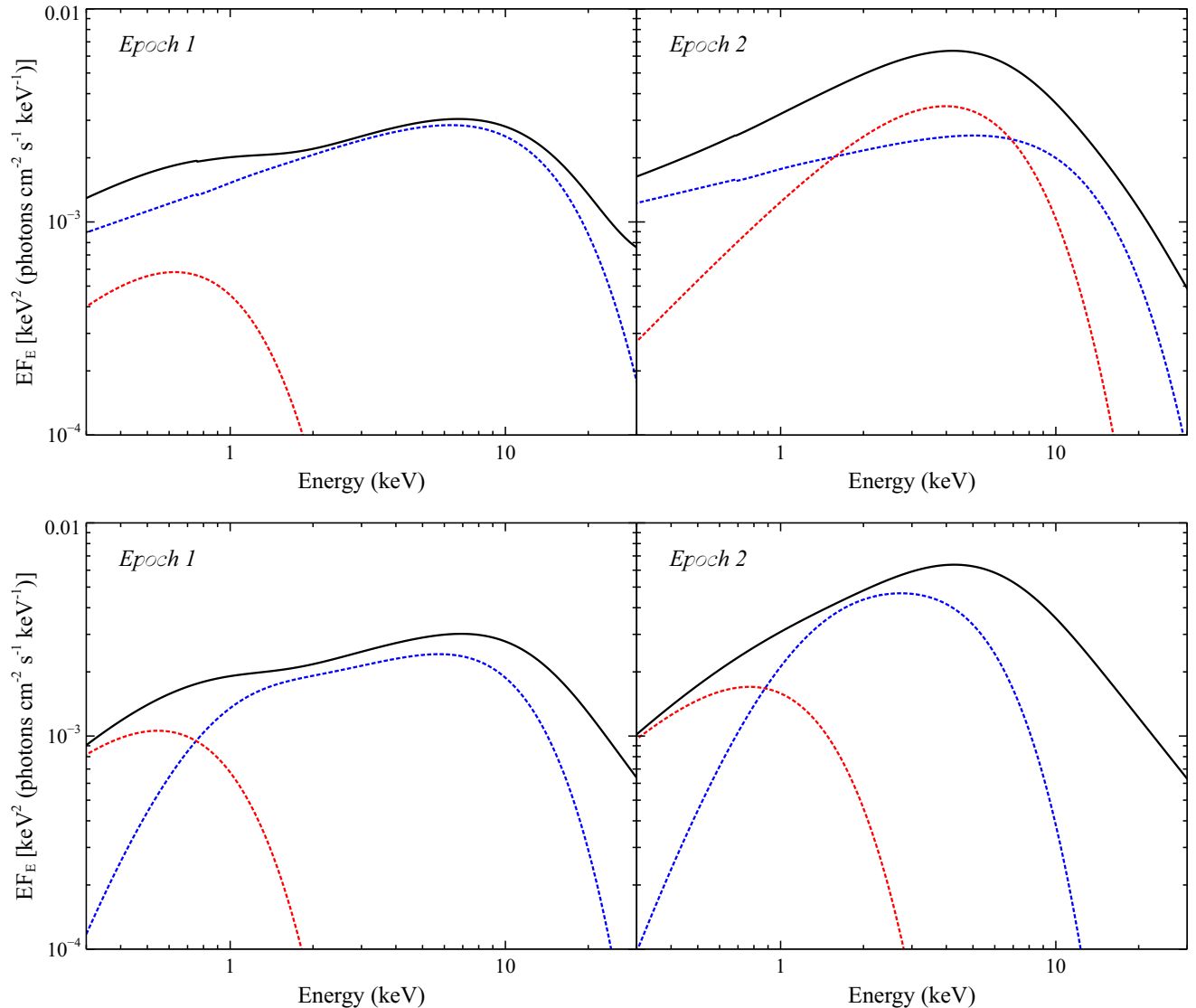
FIG. 9.— Top panels: the relative contribution of the various spectral components inferred with the DISKBB+SIMPL \otimes DISKPBB model (corrected for absorption) for each epoch. The full model is shown in black, while the DISKBB contribution is shown in red, and the DISKPBB contribution (before modification by SIMPL) is shown in blue. In this case, the spectral evolution is dominated by the cooler of the two thermal components (represented by DISKBB). Bottom panels: The same as the top panels, but for the DISKBB+SIMPL \otimes COMPTT model. Here, the DISKBB contribution is shown in red, and the COMPTT contribution (before modification by SIMPL) is shown in blue. In this case, the spectral evolution is dominated by the hotter of the two thermal components (represented by COMPTT).
