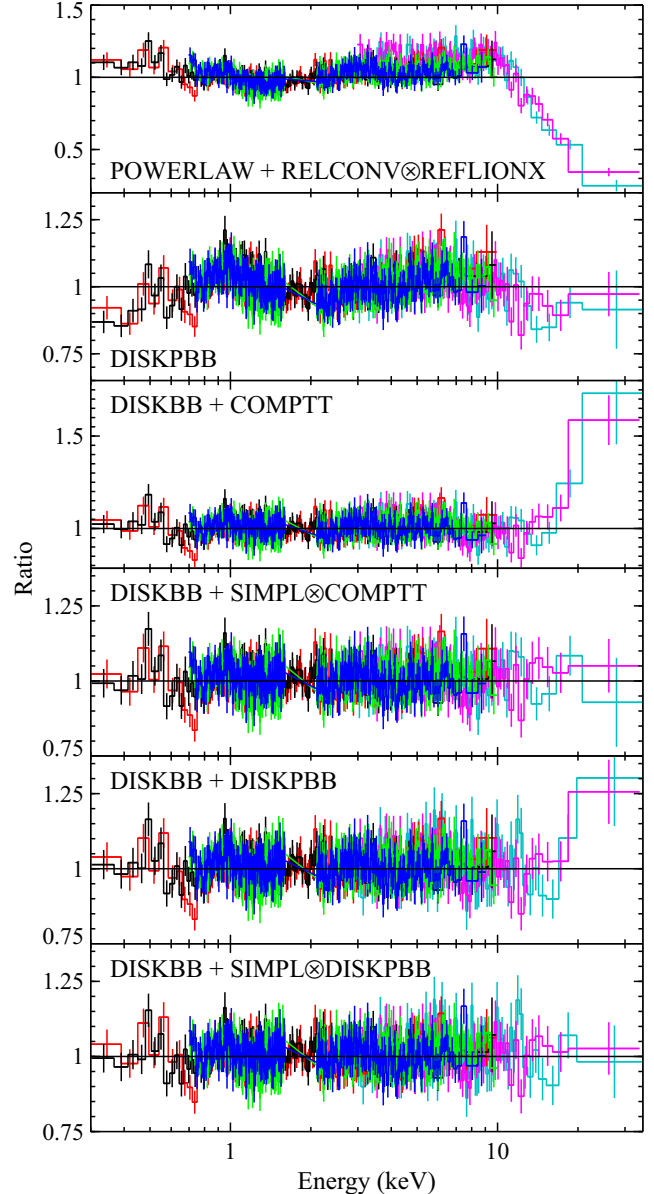
FIG. 5.— Data/model ratios for a variety of the continuum models applied to the full broadband X-ray spectrum of Holmberg IX X-1 obtained during epoch 1 (see section 3.1.2). The color scheme is the same as for Figures 3 and 4, and the data have again been rebinned for visual clarity.
