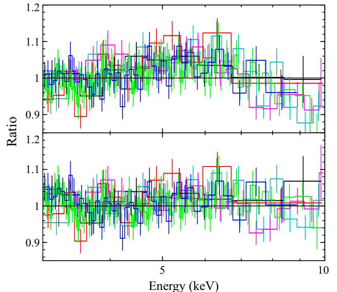
FIG. 3.— Data/model ratios for the XMM-Newton (black: EPIC -pn, red: EPIC -MOS), Suzaku (green: FI XIS, blue: BI XIS) and NuSTAR (magenta: FPMA, cyan: FPMB) datasets obtained during epoch 1, modelled with both a powerlaw continuum ( top panel ) and a bremsstrahlung continuum ( bottom panel ). The data from the various missions display consistent curvature across their common energy range (3–10 keV). The data have been rebinned for visual clarity.
