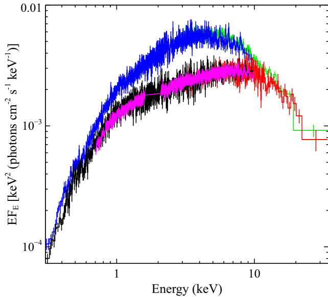
FIG. 6.— The spectral evolution displayed by Holmberg IX X-1 between the two epochs. The XMM-Newton ( EPIC -pn), Suzaku (FI XIS) and NuSTAR (FPMA) data from epoch 1 are shown in black, magenta and red, respectively, while the XMM-Newton and NuSTAR data from epoch 2 are shown in blue and green. All the data have been unfolded through the same model, which again consists of a constant.
