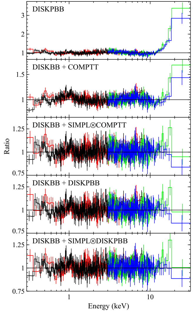
FIG. 7.— Data/model ratios for a variety of the continuum models applied to the full broadband X-ray spectrum of Holmberg IX X-1 obtained during epoch 2 (see section 3.2). XMM-Newton EPIC -pn and EPIC -MOS data are shown in black and red, respectively, and NuSTAR FPMA and FPMB in green and blue; the data have been rebinned for visual clarity.
