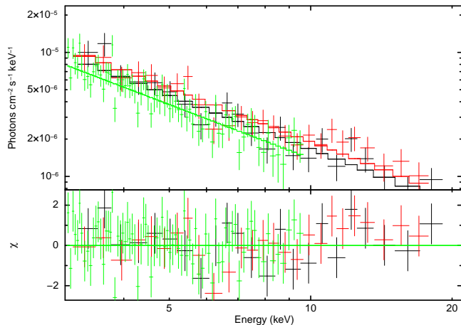
Figure 2. Unfolded 3-20 keV NuSTAR + XMM-Newton EPIC-PN spectra of the Geminga pulsar fit with a single power-law model. The green, black and red data points are for XMM-Newton EPIC-PN, NuSTAR FPMA and FPMB, respectively.
