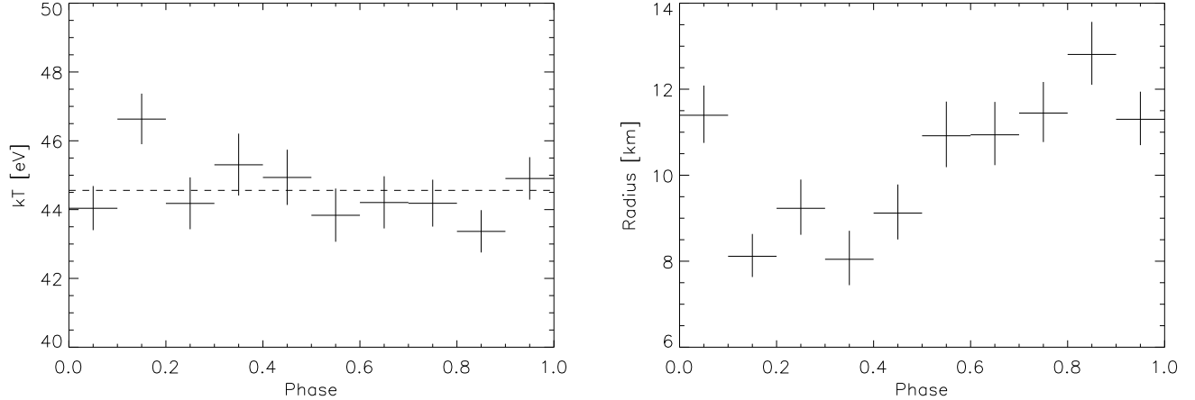
Figure 7. Phase variation of the fitted blackbody temperature (left) and radius at d = 250 pc (right). XMM-Newton data in the 0.25–10 keV band were used for spectral fitting. The phase zero is identical to that of the folded lightcurves in Figure 6.
