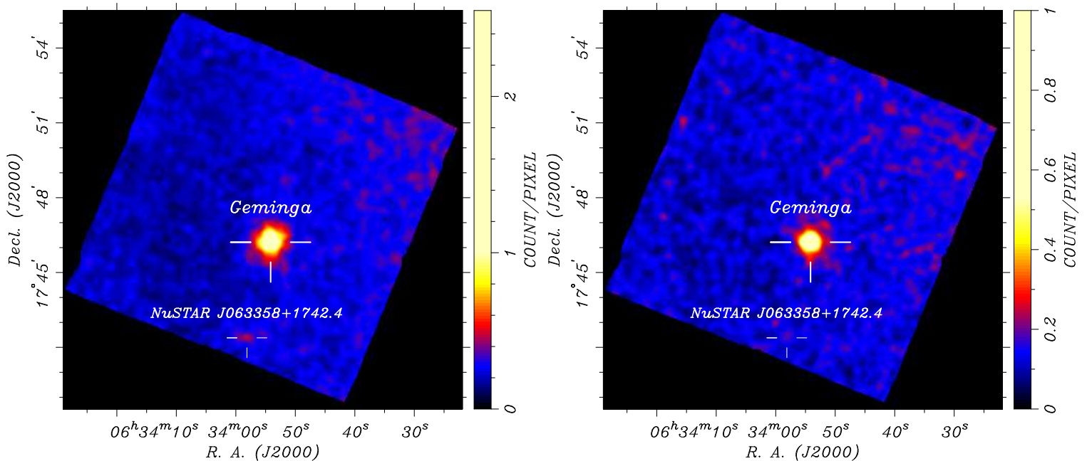
Figure 1. NuSTAR mosaic image of the field containing Geminga pulsar, in the 3-10 keV (left) and 10-20 keV (right) bands. Data from all Geminga NuSTAR observations and modules are merged, with appropriate exposure corrections applied. The locations of Geminga and NuSTAR J063358+1742.4, as determined using wavedetect , are indicated by the tick marks.
