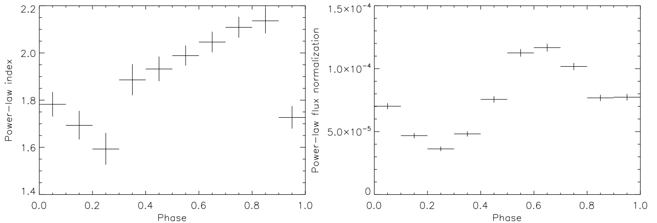
Figure 8. Phase variation of the best-fit power-law index (left) and flux normalization [ \text{ph cm}^{-2} \text{s}^{-1} \text{keV}^{-1} ] at E = 1 keV (right) in the 0.25–10 keV band. XMM-Newton data in the 0.25–10 keV band were used for spectral fitting. The phase zero is identical to that of the folded lightcurves in Figure 6.
