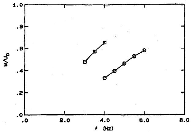
Fig. 11 Estimate of the magnitude of the axial velocity along vortex cores.
