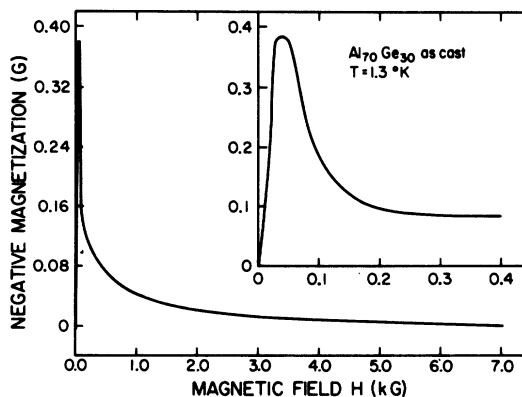
FIG. 7. Magnetization as a function of magnetic field for cast \text{Al}_{70}\text{Ge}_{30} at 1.3^\circ\text{K} . The insert shows the low-field data.
