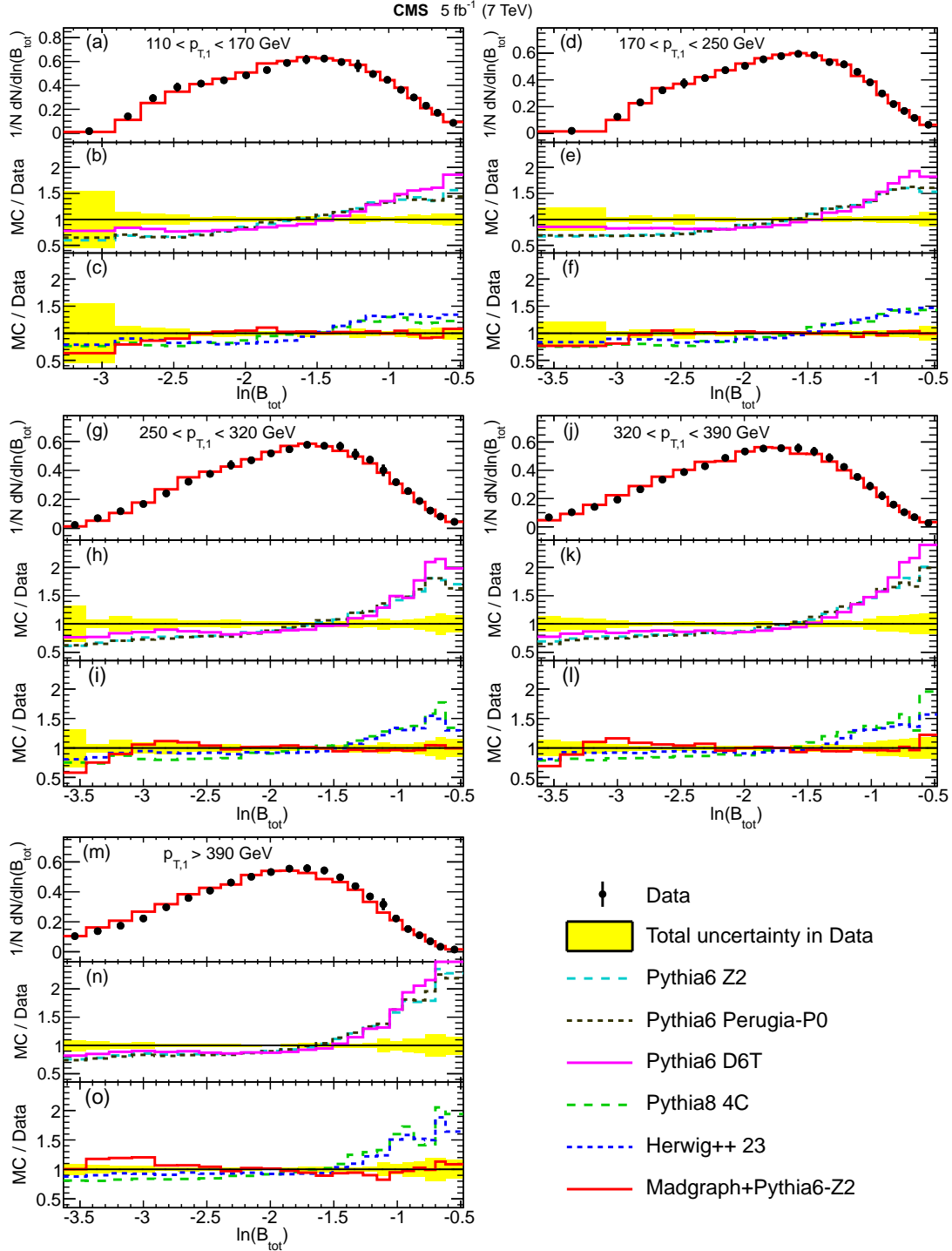
Figure 2: Comparison between the jet broadening B_{\text{tot}} distributions in data and various Monte Carlo models. The p_T bins and other details are the same as in Fig. 1.
