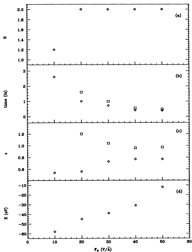
FIG. 5. Ionization properties of beryllium as a function of F_0 for \omega = 5 \text{ fs}^{-1} : (a) average number of electrons ( N ) ionized in 5 fs, (b) average time of ionization of the first electron (diamonds) and the second electron (squares), (c) \epsilon of the first electron to ionize (diamonds) and the second electron to ionize (squares), and (d) total energy of the core ( E ) at the time the second electron ionizes.
