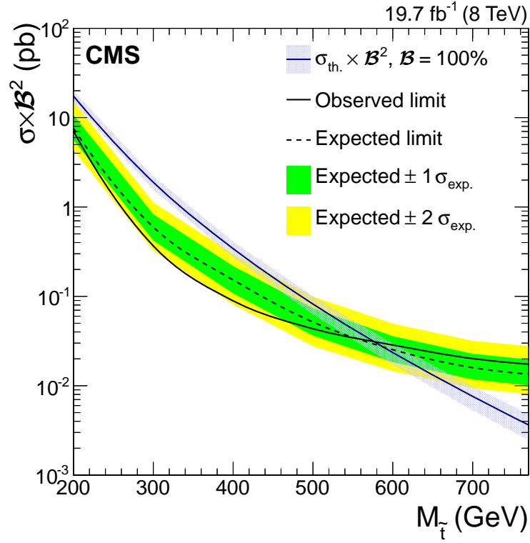
Figure 4: The expected and observed combined upper limits on the top squark pair production cross section \sigma times the square of the branching fraction, \mathcal{B}^2 , at 95% CL, as a function of the top squark mass. These limits apply to top squarks with a chargino-mediated decay through the coupling \lambda'_{3kj} . The green (darker) and yellow (lighter) uncertainty bands represent 68% and 95% CL intervals on the expected limit. The dark blue curve and the hatched light blue band represent the theoretical top squark pair production cross section, assuming \mathcal{B} = 100\% , and the uncertainties due to the choice of PDF and renormalization/factorization scales.
