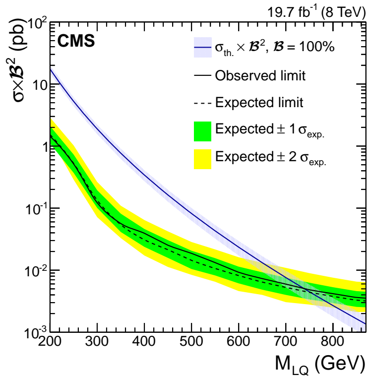
Figure 3: The expected and observed combined upper limits on the third-generation LQ pair production cross section \sigma times the square of the branching fraction, \mathcal{B}^2 , at 95% CL, as a function of the LQ mass. These limits also apply to top squarks decaying directly via the coupling \lambda'_{333} . The green (darker) and yellow (lighter) uncertainty bands represent 68% and 95% CL intervals on the expected limit. The dark blue curve and the hatched light blue band represent the theoretical LQ pair production cross section, assuming \mathcal{B} = 100\% , and the uncertainties due to the choice of PDF and renormalization/factorization scales.
