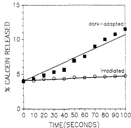
Figure 2. Time-dependent efflux of calcein from unilamellar vesicles of EYPC, pH 7.55: (O) EYPC treated with irradiated 4 ; (■) EYPC treated with dark-adapted 4 . Details of sample preparation and methods of determining rates of dye release are given in ref 12.
