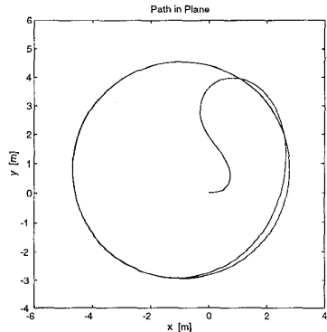
Figure 3: Resulting path in the ground plane for tracking a constant roll angle.
