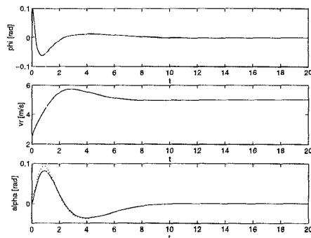
Figure 7: The steering angle (top), rear-wheel velocity v_r (middle), and roll angle \alpha (bottom) for the lane-change. The dotted curve is \alpha_* .
