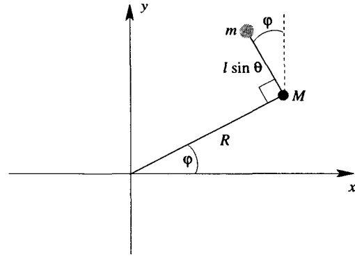
Figure 5.2: Looking down on on the whirling pendulum.
