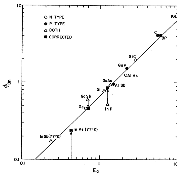
FIG. 1. Barrier heights (measured from the conduction band edge) for zincblende materials as a function of band gap. The corrected values were determined by subtracting the first-order perturbation energy from the measured value. (See text.)
