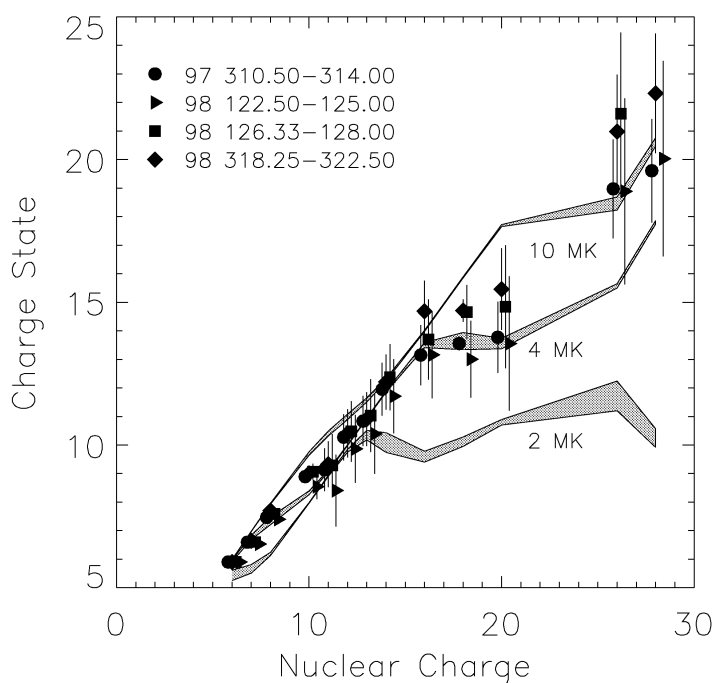
Figure 2: Inferred charge states for the four events. The shaded regions correspond to expected values for different coronal temperatures (see text).
