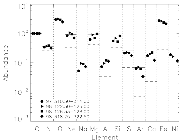
Figure 1: Abundances normalized to C for the four events. Solid (dashed) lines indicate average values for impulsive (gradual) values from Reames (1995).
