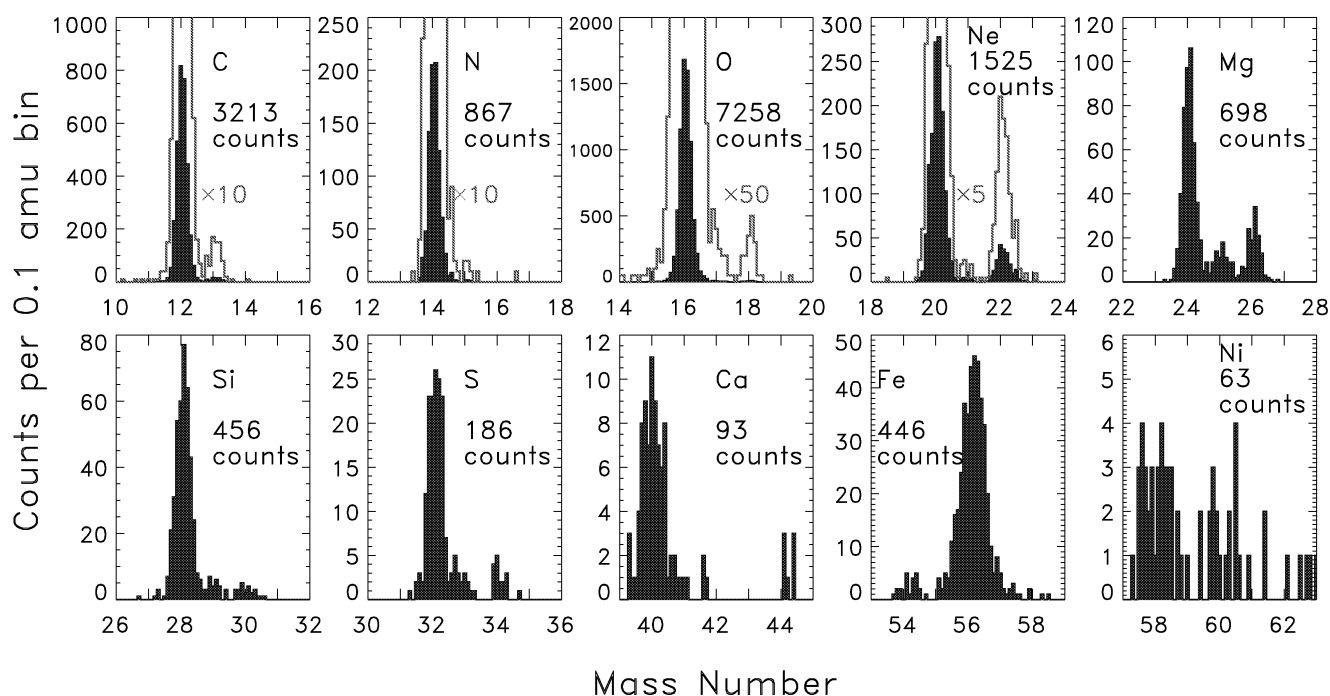
Figure 1: Mass histograms ( shaded ) from SIS, accumulated from 11/14/98 5:00 to 11/16/98 0:00. Views expanded by the factors indicated ( solid lines ) are also shown.
