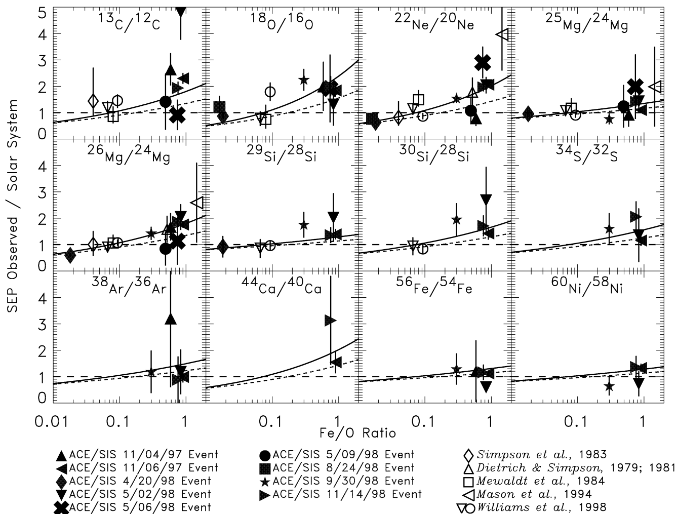
Figure 2: The isotope abundance ratios normalized to solar system values plotted vs. the observed Fe/O ratios. Preliminary values for ACE/SIS data ( filled symbols ) are from the indicated SEP events, with references for other data ( open symbols ) given in the legend. The dotted and solid curves show possible expected correlations for the ratios (see text). The dashed line indicates no deviation from the standard solar system values (Anders & Grevesse, 1989).
