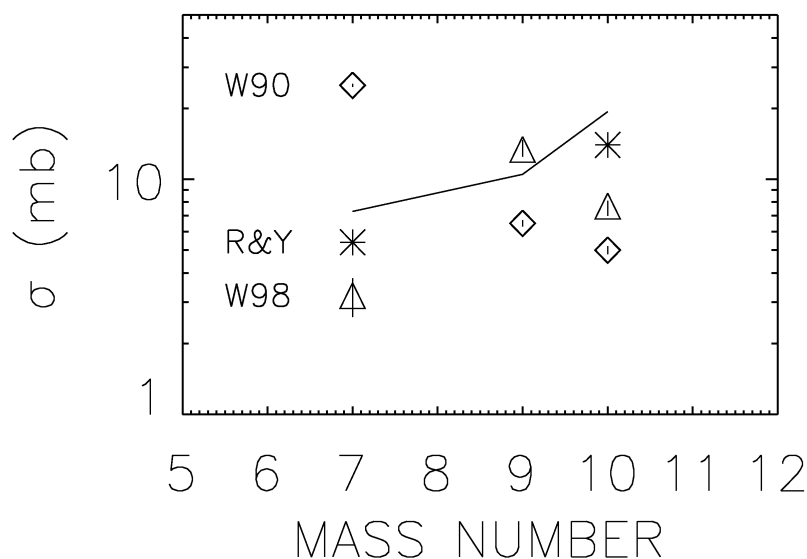
Figure 1: Isotopic yield of Be from ^{11}\text{B} at energies near 600 MeV/nucleon.
