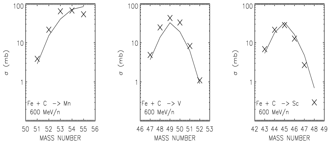
Figure 2: Yields of Sc, V, and Mn from Fe on C collisions at 600 MeV/nucleon.
