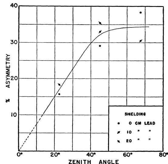
FIG. 1. The west excess in percent as a function of zenith angle with and without lead absorber.
