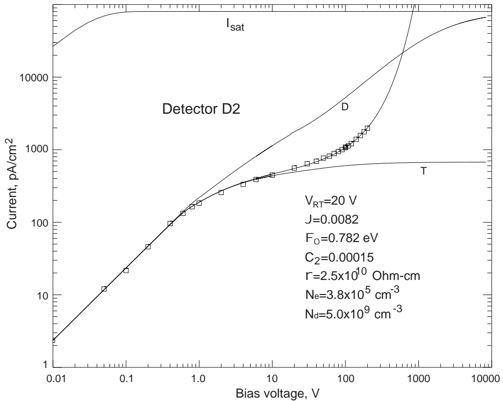
Figure 8. Same as Fig. 7 but plotted for the D2 detector.
