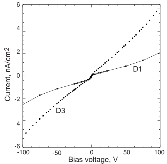
Figure 6. Comparison between representative I - V curves measured for the D1 and D3 detectors.
