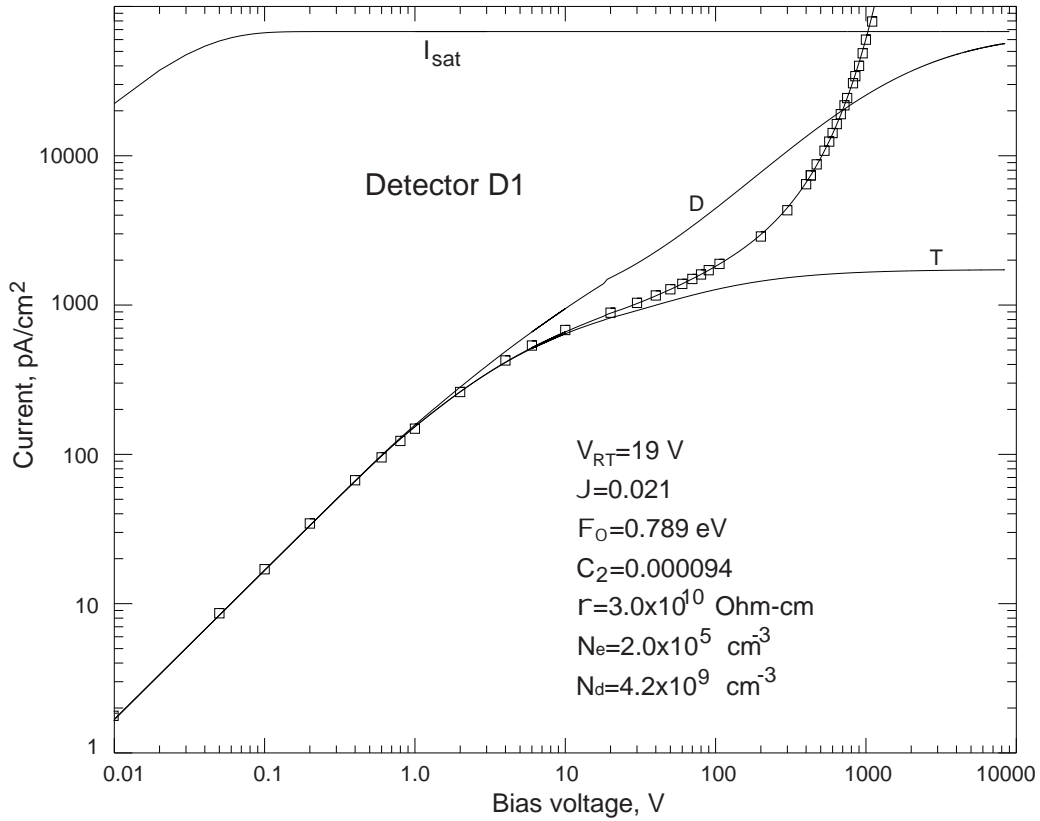
Figure 7. The measured (squares) and calculated (solid lines) I - V characteristics of the D1 detector. The curve labeled D is calculated for \vartheta_n=1 and C_2=0 (no interfacial layer), while the curve labeled T is calculated for \vartheta_n \neq 1 and C_2=0 (no potential barrier lowering). The curve I_{SAT} represents the saturation current of the ideal Schottky barrier in the termionic approximation.
