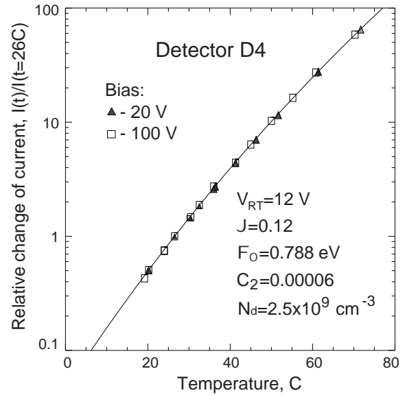
Figure 11. The temperature dependence of the dark current measured (squares) and calculated (solid lines) for 20 and 100 V biases on the cathode.
