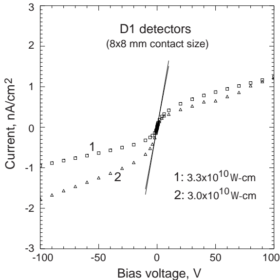
Figure 3. I - V characteristic measured for two D1 detectors. The contact size is 8x8 mm; the gap between the contact and the guard ring is 200 \mu m; the effective contact area used to normalize the current is 0.672 cm 2 .
