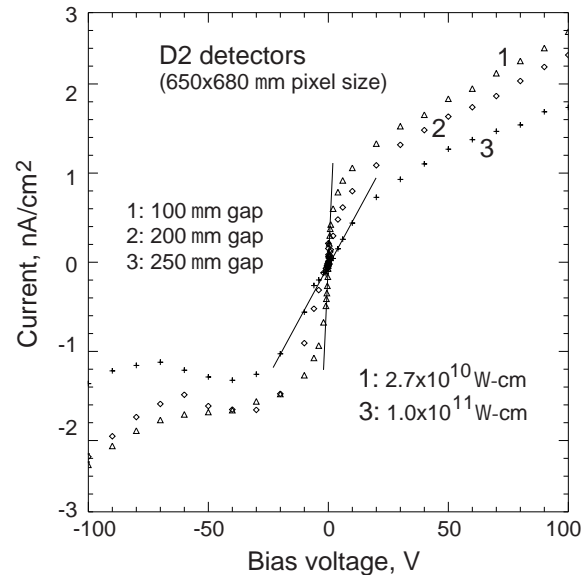
Figure 4. I - V characteristic measured for three D2 detectors; the pixel size is 650x680 \mu m; the gaps between the contact and the guard ring (grid) in \mu m are: (1) 100, (2) 200, (3) 250. The effective contact areas used to normalize the current in cm 2 are (1) 0.00264, (2) 0.00171, and (3) 0.00132.
