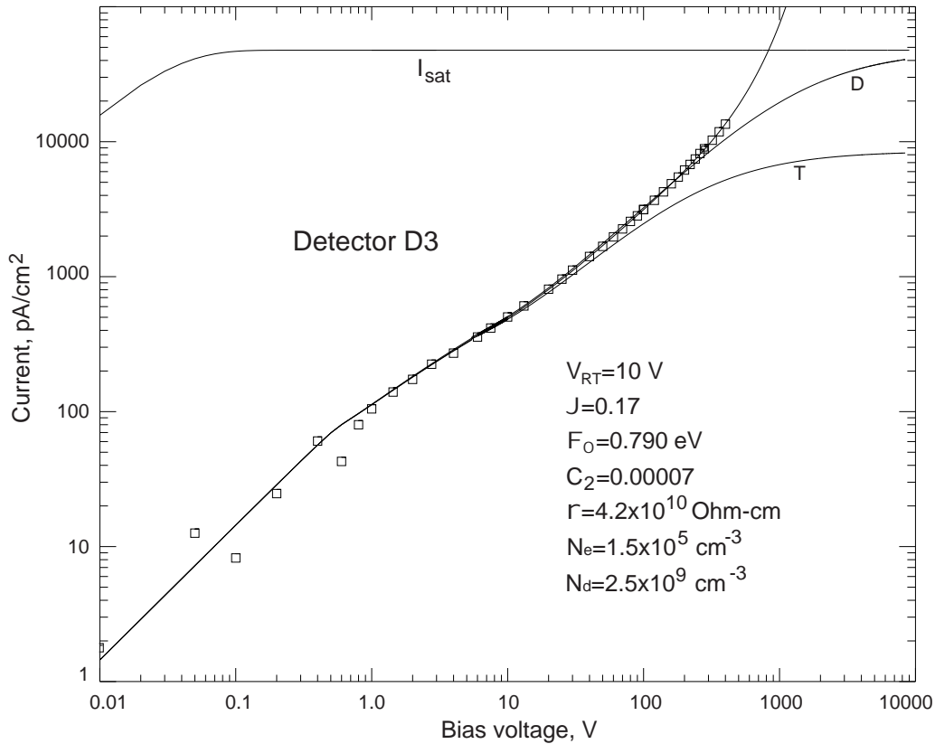
Figure 9. Same as Fig. 7 but plotted for the D3 detector.
