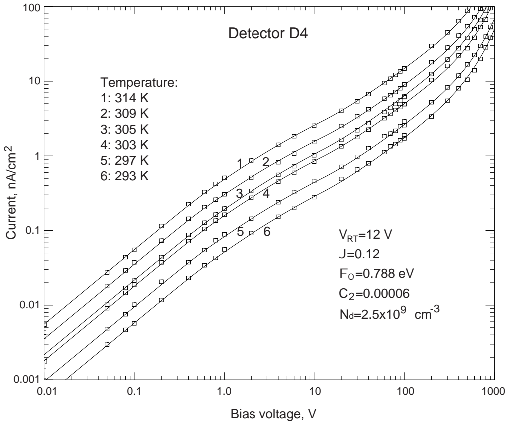
Figure 10. The measured (squares) and calculated (solid lines) I - V characteristics of a D4 detector at six detector temperatures. The same set of free parameters was used to calculate the theoretical curves for each temperature.
