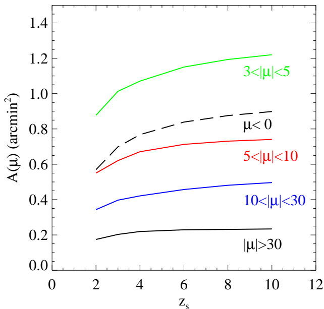
FIG. 12.— Values of the area A on the lens plane where the magnification factor \mu is included in the specified ranges for different source redshifts z_s (see also Table 6).
