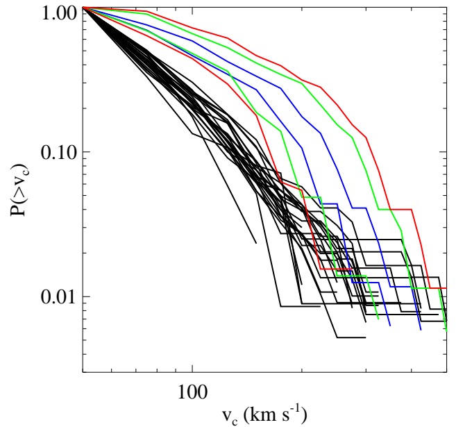
FIG. 21.— Subhalo velocity functions, i.e., probability distribution functions of subhalos with circular velocities larger than fixed values, of massive galaxy clusters estimated from cosmological simulations and our strong lensing modeling. The simulated (in black) and observed (in color) functions, measured within a two-dimensional aperture of 420 kpc, are normalized to their corresponding values at 50 \text{ km s}^{-1} . The 1\sigma , 2\sigma , and 3\sigma confidence levels, according to the best-fitting 2PIEMD + 175(+1)dPIE ( M_T L^{-1} \sim L^{0.2} ) model of MACS 0416, are shown in blue, green, and red, respectively.
