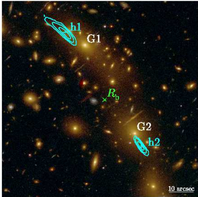
FIG. 14.— An 80'' \times 80'' cluster-core image showing the positions of the centers of the two extended dark-matter halos (h1 and h2, cyan plus symbols, see also Table 7) and of the cluster barycenter ( R_b , green cross, defined in Eq. (21)) of the best-fitting lens model. Given the uncertainties shown in Figure 13, reproduced here with cyan contours, the dark-matter-halo centers are offset from the luminosity centers of the closest brightest cluster galaxies (G1 and G2) at more than 3\sigma CL. North is up and East is left.
