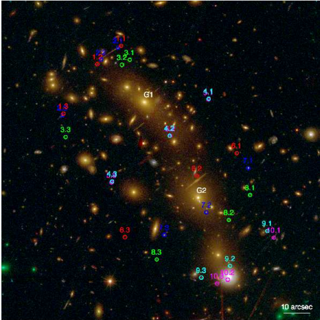
FIG. 1.— A 2' \times 2' color-composite image of MACS J0416.1–2403 obtained by combining the 16 filters of HST /ACS and WFC3. North is top and East is left. The thirty multiple images modeled in this paper and the two brightest cluster galaxies, G1 and G2, are labeled. More information about these objects is provided in Tables 1 and 3 and Figure 2.
