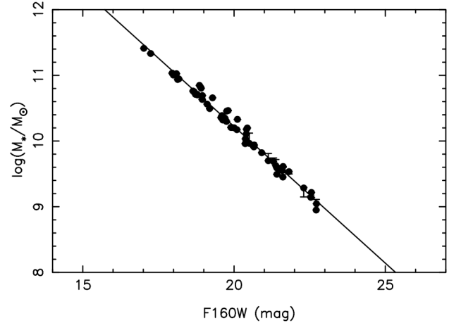
FIG. 7.— Best-fitting stellar mass values, obtained from the SED modeling of the multicolor HST photometry, as a function of the magnitude values measured in the reddest HST /WFC3 broadband (F160W). The points, with 1\sigma error bars, represent 63 spectroscopically confirmed galaxy cluster members. The solid line shows the best-fitting line.
