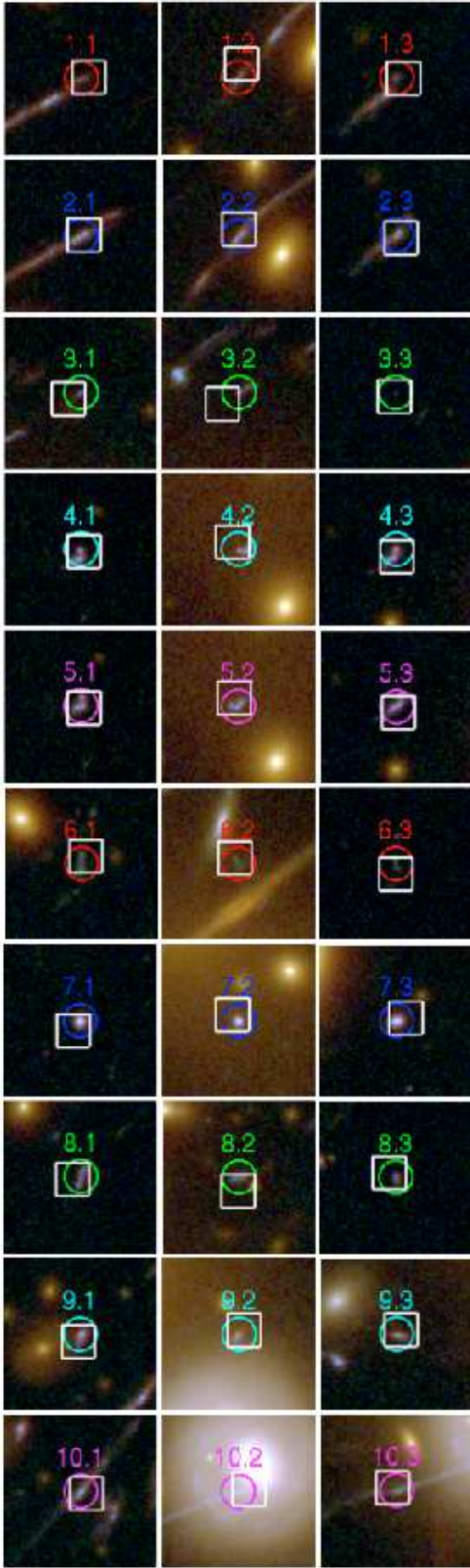
FIG. 8.— Snapshots (6 arcsec across) of the 10 strong lensing systems with spectroscopic redshifts. The observed and predicted (by the best-fitting model, see Table 5) positions of the multiple images are marked, respectively, with colored circles and white squares.
