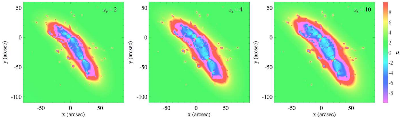
FIG. 11.— Magnification maps in the inner regions of MACS 0416 reconstructed from the best-fitting strong lensing model (see Table 5) for sources at redshifts z_s equal to 2 ( on the left ), 4 ( in the middle ), and 10 ( on the right ). The different colors, as indicated by the color bar on the right side, represent the different values of the magnification factor \mu on a linear scale extending from -10 to 10 .
