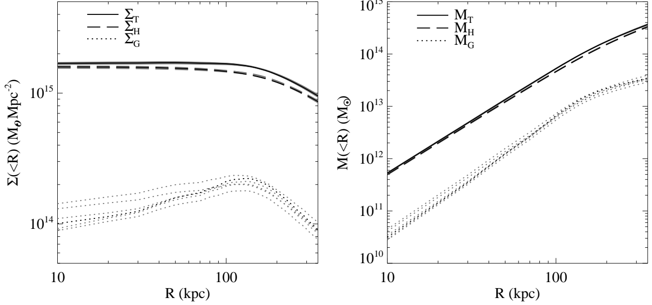
FIG. 17.— Surface mass density, \Sigma(<R) , and cumulative projected mass, M(<R) , profiles of the six optimized strong lensing models that include the 175 candidate cluster members (see Table 5). The 2PIEMD + 175(+1)dPIE ( M_T L^{-1} \sim L^{0.2} ) model is shown in black, all the others in gray. The solid, long-dashed, and dotted lines represent, respectively, the best-fitting total, cluster dark-matter halo, and cluster member profiles of the different models.
