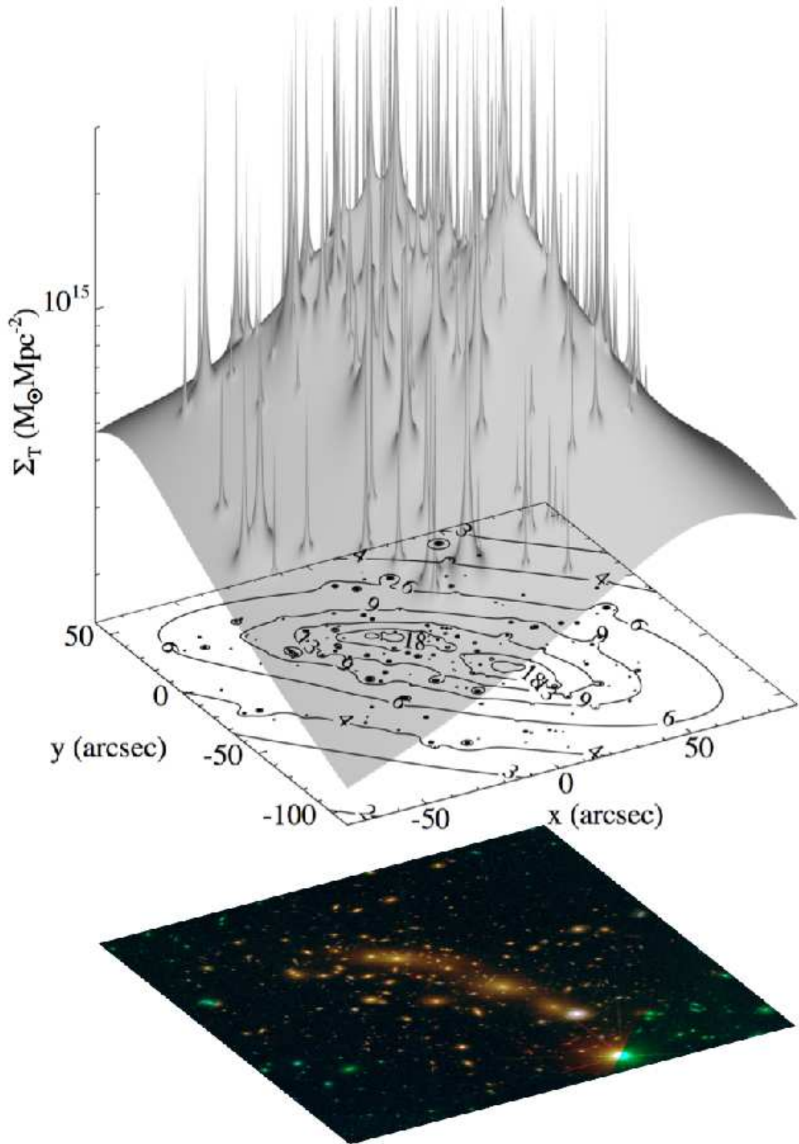
FIG. 9.— The total surface mass density \Sigma_T in the inner regions of MACS 0416 reconstructed from the best-fitting strong lensing model (see Table 5). The different contributions of the two extended dark-matter halo and many candidate cluster member components are visible. The contour levels on the lens plane are in units of 10^{14} M_\odot \text{Mpc}^{-2} .
