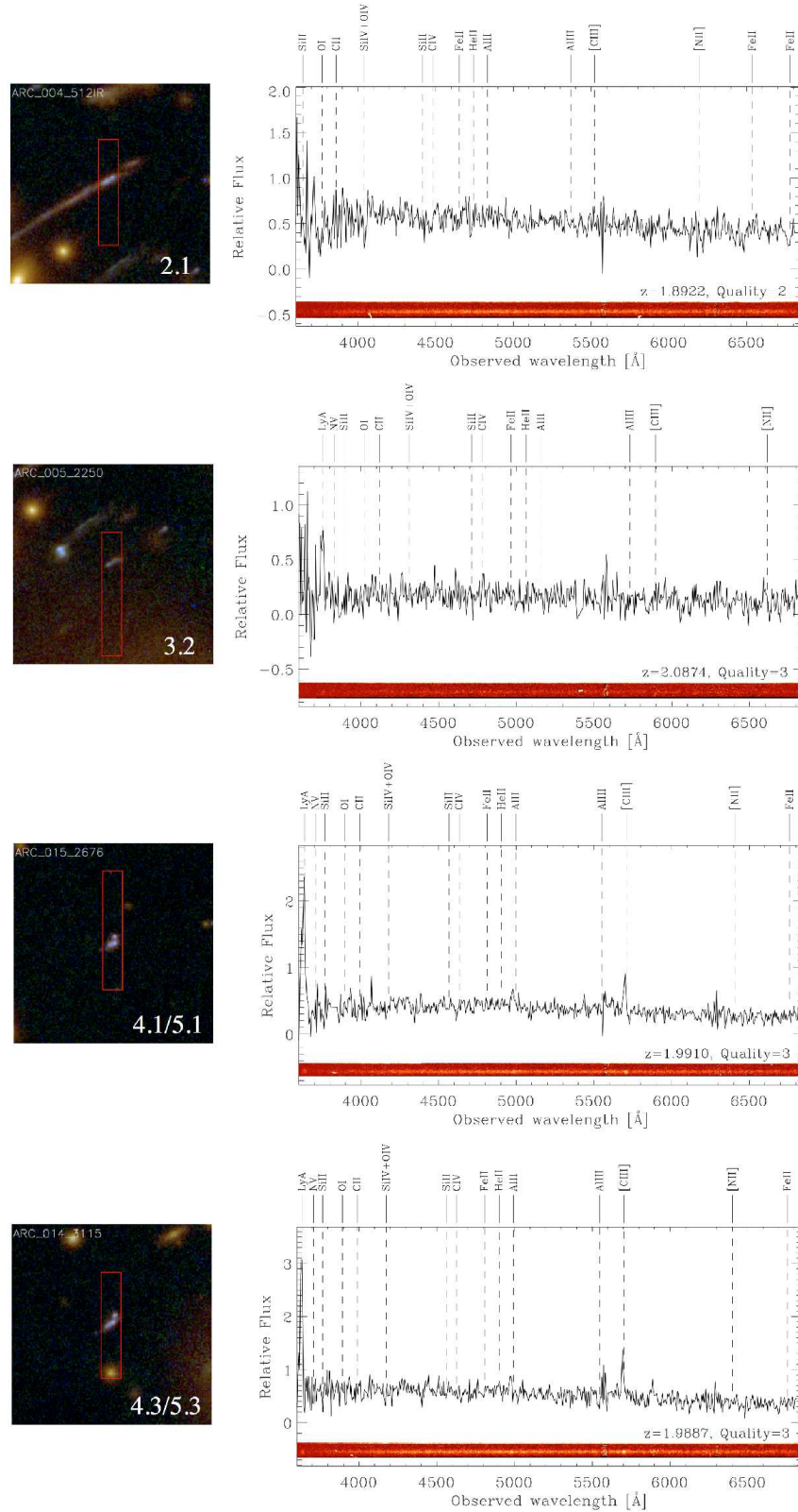
FIG. 2.— VLT/VIMOS slits and spectra of the multiple image systems. For each lensed image, we show, on the left, a multi-color HST snapshot with the VIMOS 1'' -wide slit position and orientation (in red) and the associated ID from Table 3 and, on the right, the 1D and 2D spectra with the estimated redshift value and spectroscopic quality flag (see Section 2.2). The main emission and absorption lines of a template shifted to the measured redshift value are also indicated.
