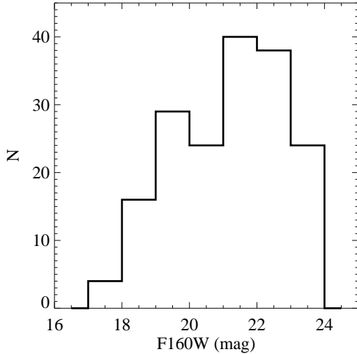
FIG. 5.— Histogram of the near-IR F160W magnitudes of the 175 candidate cluster members shown in Figure 4.
