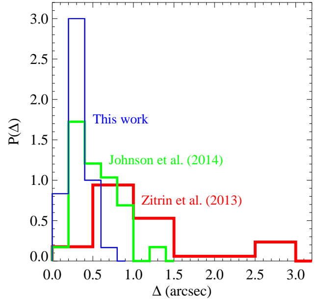
FIG. 19.— Probability distribution functions of the absolute values of the differences ( \Delta , in arcsec) between the observed and best-fitting model-predicted positions of the multiple-image systems considered in the different strong lensing studies of MACS 0416.
