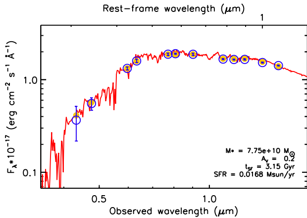
FIG. 6.— Example of the composite stellar population modeling of the 12 reddest HST bands of a spectroscopically confirmed galaxy cluster member. We use Bruzual & Charlot (2003) templates (the best-fitting one is shown here in red) at solar metallicity, with dust and a Salpeter stellar IMF. Observed fluxes with 1\sigma errors are represented with blue empty circles and bars, model-predicted fluxes are shown as orange filled circles.
