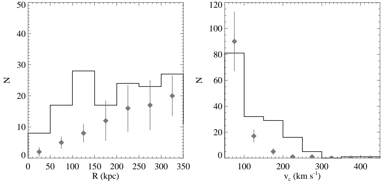
FIG. 22.— Number of subhalos as a function of the projected distance from the galaxy cluster center ( on the left ) and, within a two-dimensional aperture of 420 kpc, of their circular velocity value ( on the right ). The black histograms represent the values derived in our analysis of MACS 0416 and the gray diamonds and bars show, correspondingly, the median values and the 1\sigma uncertainties obtained from cosmological simulations.
