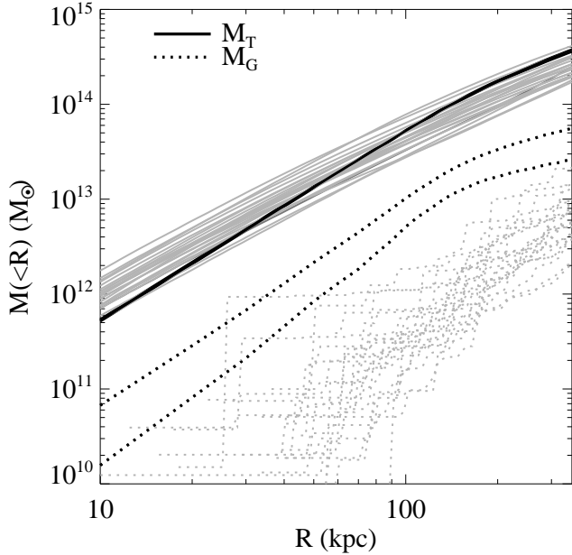
FIG. 20.— Cumulative projected mass, M(<R) , profiles from the best-fitting strong lensing model of MACS 0416 (in black) and from dark-matter-only cosmological simulations of galaxy clusters (in gray). The solid and dotted lines represent, respectively, the total and cluster member profiles, at 1\sigma confidence level for MACS 0416 and as different clusters for the simulations.
