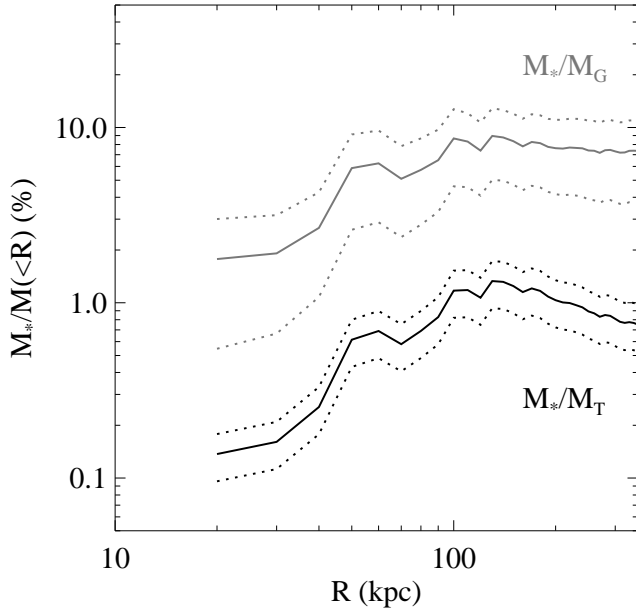
FIG. 18.— Cumulative projected profiles of the stellar over total cluster, M_*/M_T , and stellar over total galaxy, M_*/M_G , mass fractions. Solid and dotted lines show the median values and the 1\sigma confidence levels, respectively.
