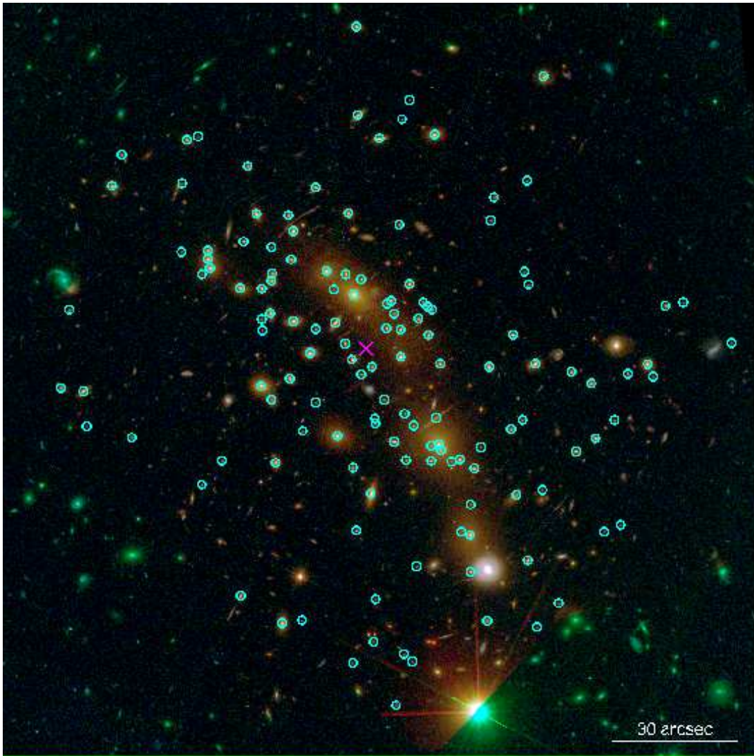
FIG. 4.— A 3' \times 3' color-composite image of MACS 0416 showing in cyan the 175 cluster members, with near-IR F160W magnitudes, selected with the method described in Section 3.3.1, based on spectroscopic and multi-color (12 bands) data, and used in the cluster strong lensing models presented in Section 3.4. The magenta cross locates the cluster luminosity center, estimated by weighting the positions of the candidate cluster members with their F160W magnitudes. North is top and East is left.
