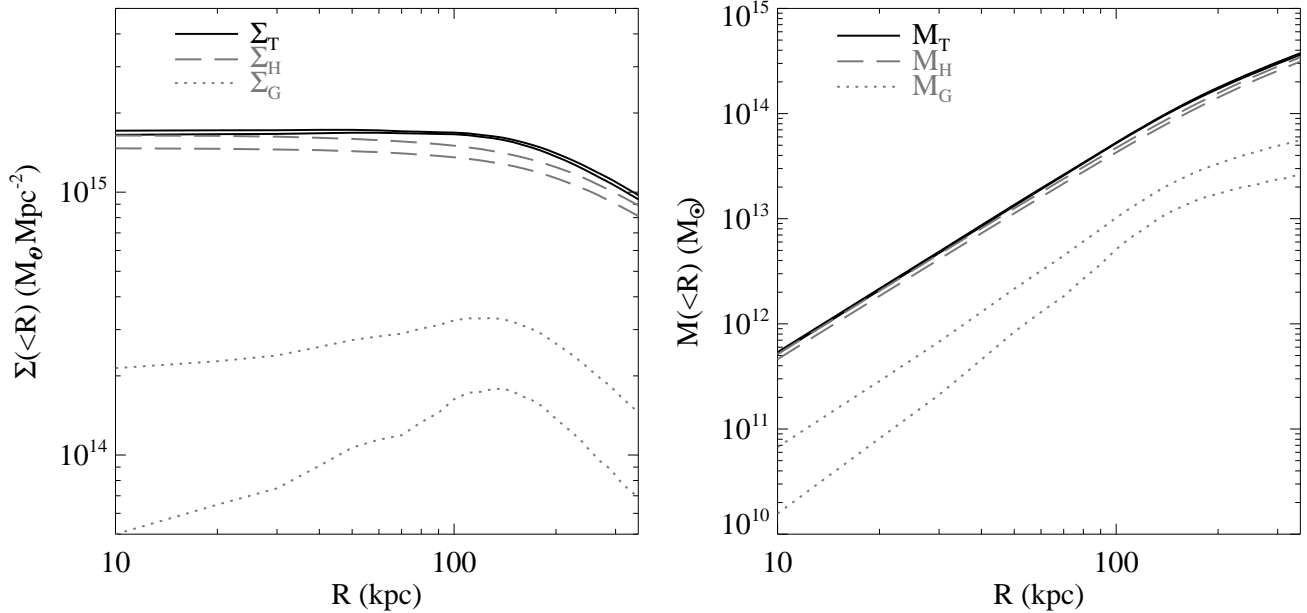
FIG. 15.— Average surface mass density, \Sigma(<R) , and cumulative projected mass, M(<R) , profiles of the 2PIEMD + 175(+1)dPIE ( M_{\text{T}}L^{-1} \sim L^{0.2} ) model. The solid, long-dashed, and dotted lines represent, respectively, the total, cluster dark-matter halo, and cluster member profiles at 1\sigma confidence level.
