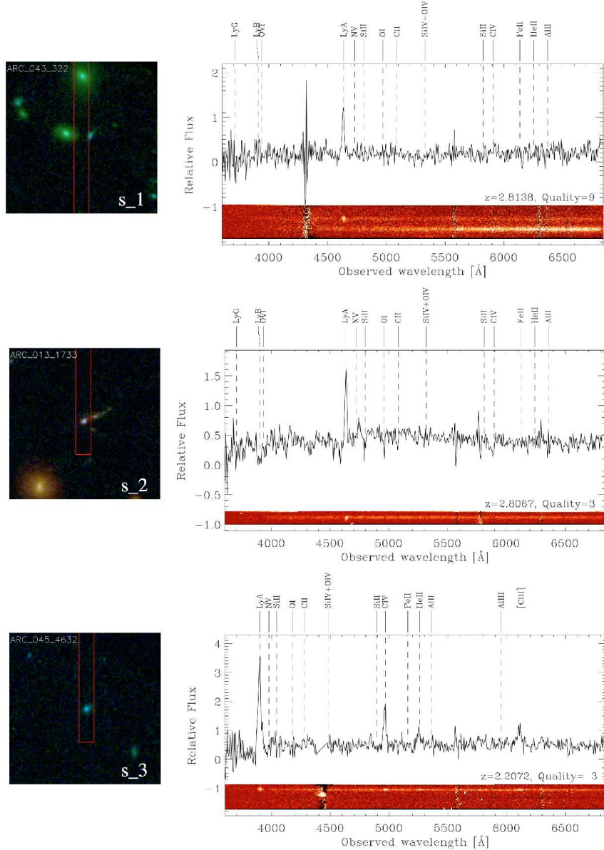
FIG. 3.— VLT/VIMOS slits and spectra of the images that are magnified but not multiply-imaged. For each magnified image, we show, on the left, a multi-color HST snapshot with the VIMOS 1'' -wide slit position and orientation (in red) and the associated ID from Table 4 and, on the right, the 1D and 2D spectra with the estimated redshift value and spectroscopic quality flag (see Section 2.2). The main emission and absorption lines of a template shifted to the measured redshift value are also indicated.
