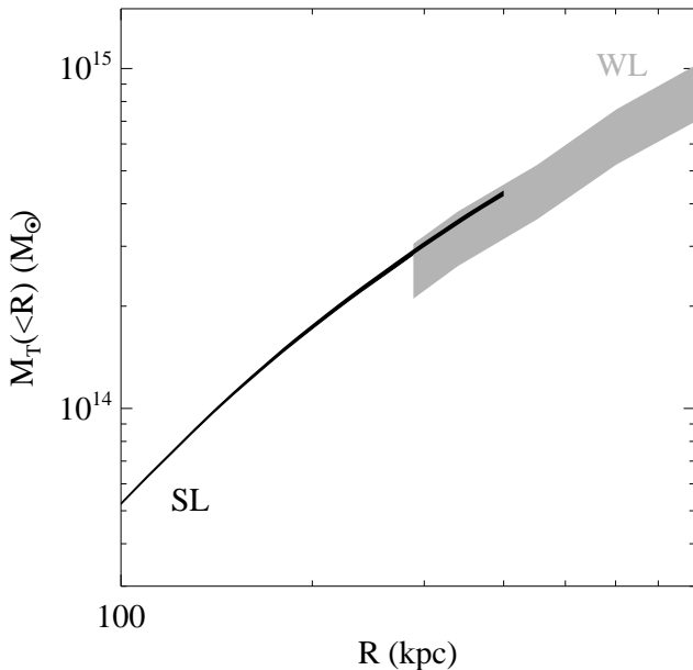
FIG. 16.— The cumulative projected total mass, M_{\text{T}}(<R) , profiles obtained from the strong lensing (SL) analysis presented in this work, i.e., from the 2PIEMD + 175(+1)dPIE ( M_{\text{T}}L^{-1} \sim L^{0.2} ) model, and from the weak lensing (WL) analysis presented in Umetsu et al. (2014). Intervals are at 1\sigma confidence level.
