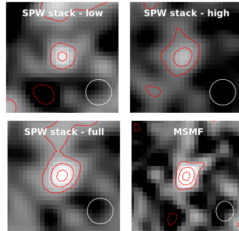
Figure 1. Cutouts of 4'' on the side centered on CID-42: low frequency SPW stack, high frequency SPW stack, full SPW stack and MSMF map. All SPW stacks have the same resolution of 0.9'' , while the MSMF map has a resolution of 0.7'' . The synthesized beam size is shown in the lower right corner of each panel. Contours of \pm 2\sigma , \pm 4\sigma and \pm 6\sigma are overplotted in red (negative contours are drawn with dashed lines). Local rms in each map is listed in Table 2.
