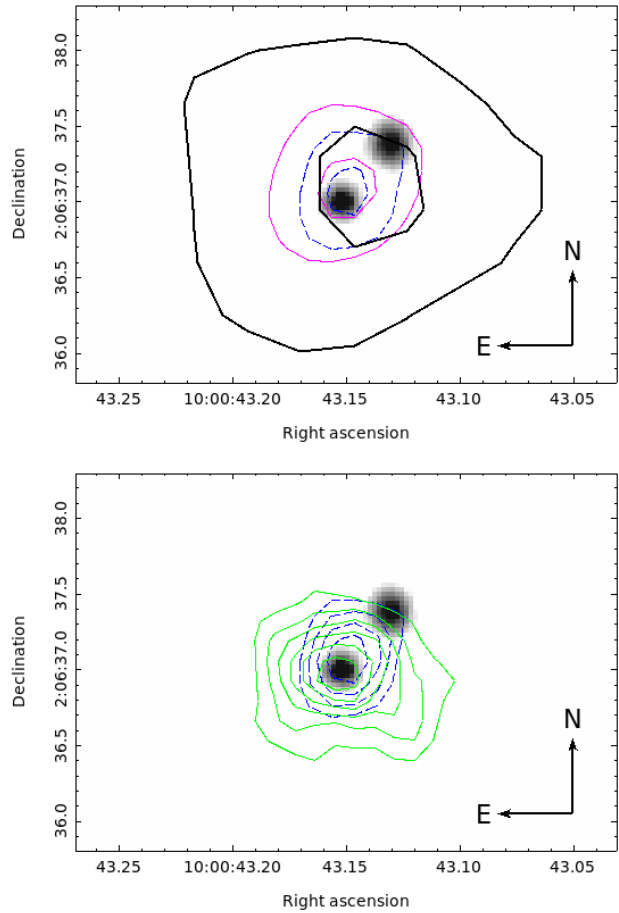
Figure 2. Top: HST/ACS gray-scale image showing the two optical components of CID-42 with contours from the radio data overlaid. For each radio map, two contour lines are shown that correspond to 3\sigma and 6\sigma . Thick black lines show data from the VLA 1.4 GHz large map from Schinnerer et al. (2007) with \sigma = 10 \mu\text{Jy beam}^{-1} . Thin magenta lines and dashed blue lines are from the VLA 3 GHz SPW stack map and MSMF map with the local rms of 4.8 \mu\text{Jy beam}^{-1} and 4.6 \mu\text{Jy beam}^{-1} , respectively. Bottom: HST/ACS gray-scale image of CID-42 with contours from the adaptively smoothed X-ray Chandra High Resolution Camera image with a 3 pixel radius Gaussian kernel by Civano et al. (2012b) in green and VLA 3 GHz MSMF map with 1\sigma steps starting from the 3\sigma in blue.
