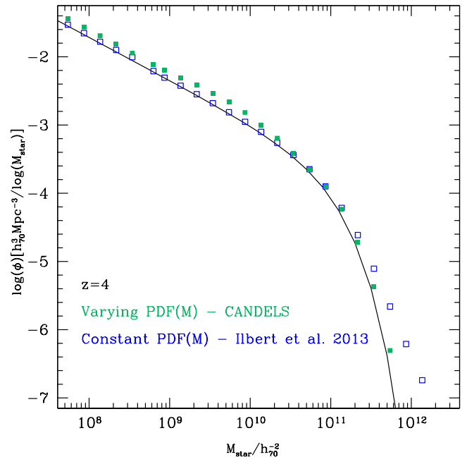
Fig. B.2. The effect of different prescription of the Eddington bias on the observed GSMF. The black line shows a Schechter function representing a GSMF with \alpha \simeq -1.6 and M_* \simeq 11 . The open blue squares show the resulting GSMF in bins of 0.2 in \log M after convolution with a constant PDF at all masses, as adopted by Ilbert et al. (2013) at z = 4 . The green filled squares represent the GSMF after convolution with the more realistic mass-dependent PDF that widens when mass decreases as we find in CANDELS (Fig.B.1).
