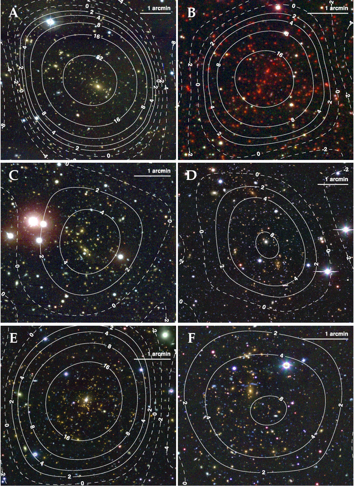
FIG. 8.— A sample of clusters from the 2500 \text{ deg}^2 SPT-SZ cluster catalog. For each cluster we display an optical/NIR rgb image with the SZ detection contours over-plotted; see §6.4 for more details on particularly notable systems. (a) SPT-CL J2248–4431 (ACO S1063; \xi = 42.4 , z = 0.351 ). This cluster is the most significant detection in the SPT sample (MPG/ESO WFI IRV -band image). (b) SPT-CL J2106–5844 ( \xi = 22.2 , z = 1.132 )—also shown in SPT mm-wave data in Figure 1—is the most massive known cluster at z > 1 . ( Spitzer /IRAC 3.6 \mu\text{m} , Magellan/FourStar J -band, Magellan/IMACS i -band image) (c) SPT-CL J0410–6343 ( \xi = 5.6 , z = 0.52 ) is a “typical” SPT cluster at approximately the median redshift and \xi of the confirmed cluster sample. (Blanco/MOSAIC-II gri -band image). (d) SPT-CL J0307–6225 ( \xi = 8.5 , z = 0.581 ) is undergoing a major merger. As SZ selection is not greatly influenced by mergers or complicated astrophysics at the cores of clusters (e.g., Motl et al. 2005, Fabjan et al. 2011), the SPT sample is representative of the entire population of massive clusters (Magellan/Megacam gri -band image). (e) SPT-CL J2344–4243 (the “Phoenix Cluster”; \xi = 27.4 , z = 0.596 ) is the most X-ray luminous cluster known. We confirm this cluster as a strong lens using newly-acquired Megacam imaging (Magellan/Megacam gri -band image). (f) SPT-CL J0307–5042 ( \xi = 8.4 , z = 0.55 ) is one of many strong-lensing clusters in the SPT sample (Magellan/Megacam gri -band image).
