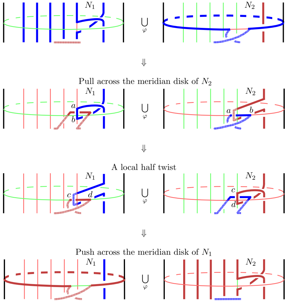
Figure 5: Local pictures of the 3-step isotopy from \beta_1 \sqcup c_2 to c_1 \sqcup \beta_2
