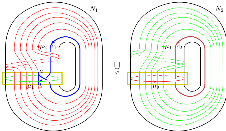
Figure 2: Writhe the core c_1 in N_1
