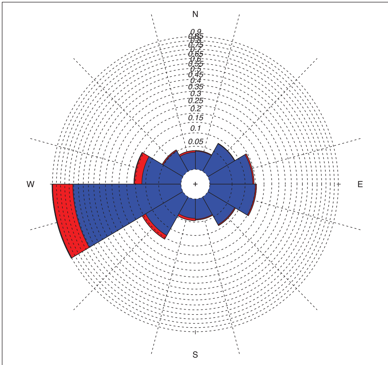
Figure S6: Windrose depicting most frequent wind direction is on-shore (westerly), with occasional reversals (from LAX, 2009-present).
